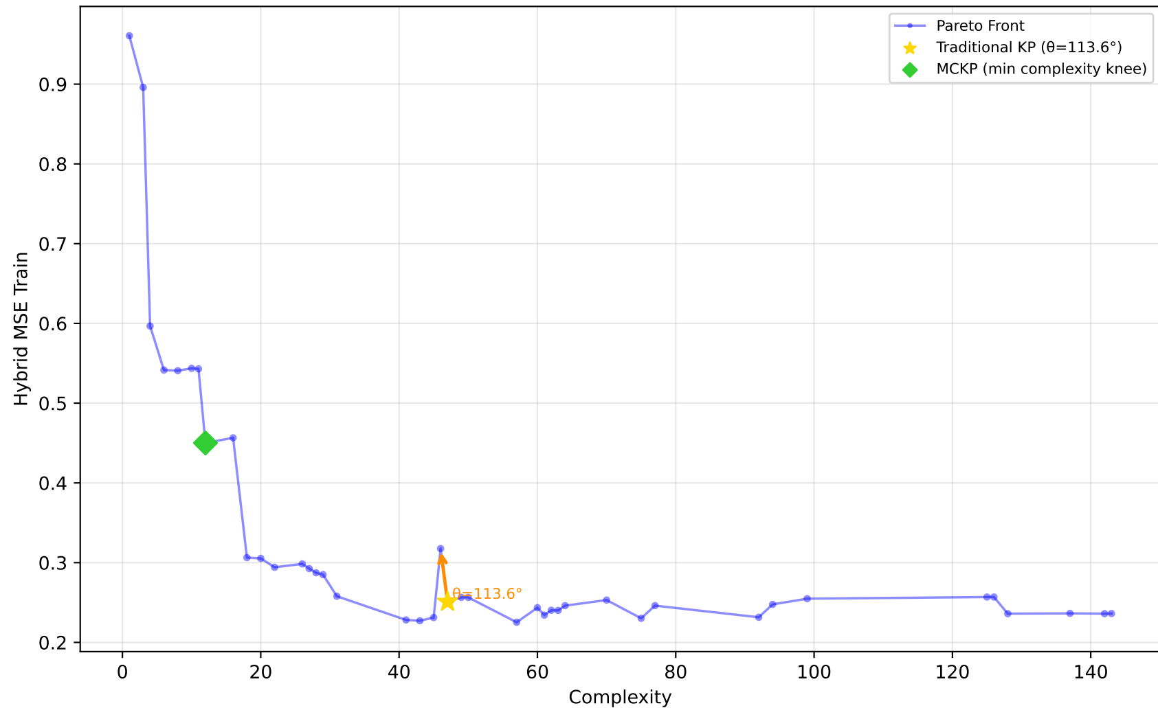
637_fri_c1_500_50 - Run 2 - SVP - Hybrid MSE Train \lambda_1=0.10, \lambda_2=0.00, \lambda_3=0.20 | Difficulty: 1.00 | Method: hmr
