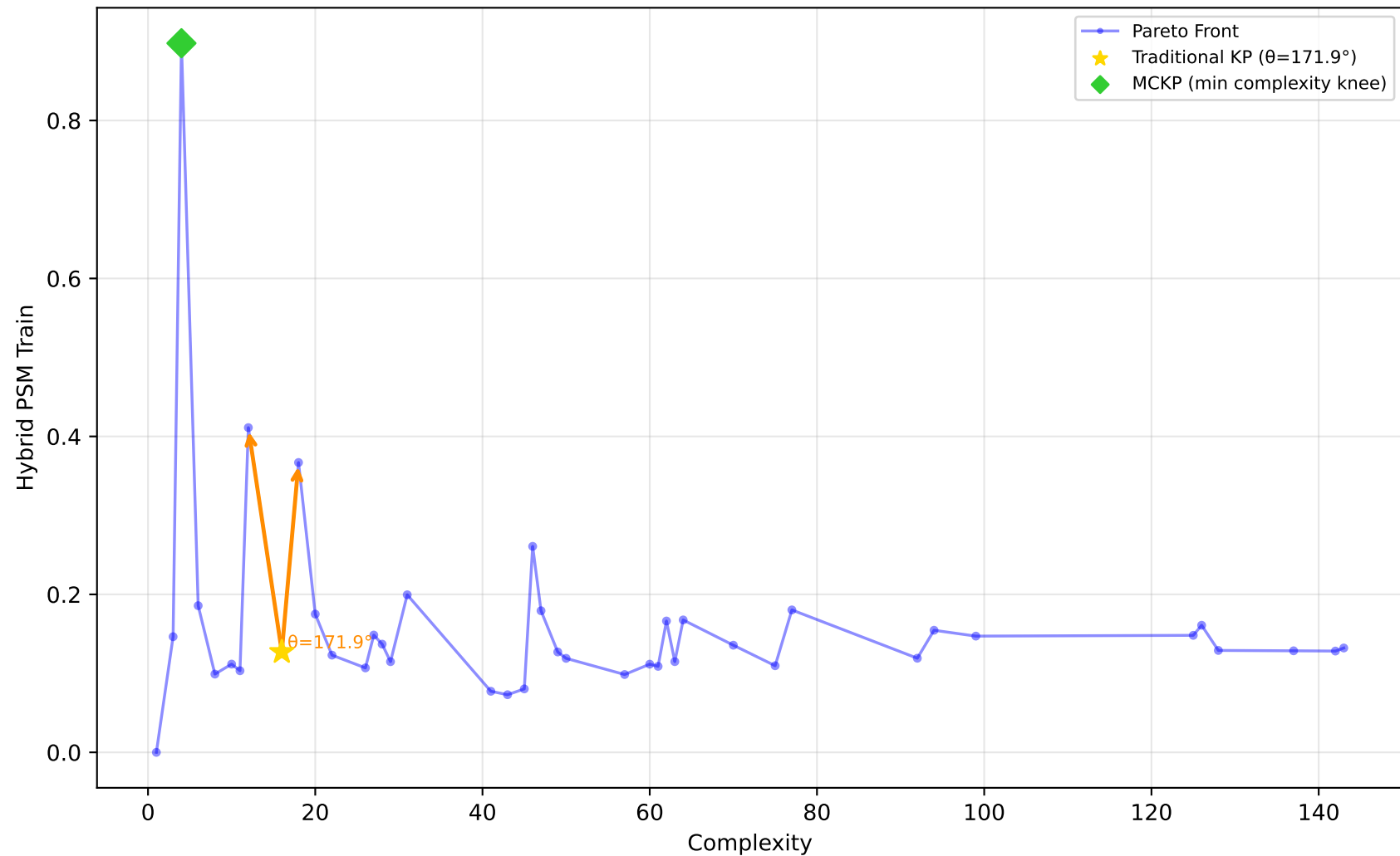
637_fri_c1_500_50 - Run 2 - SVP - Hybrid PSM Train \lambda_1=0.10, \lambda_2=0.00, \lambda_3=0.20 | Difficulty: 1.00 | Method: hmr
