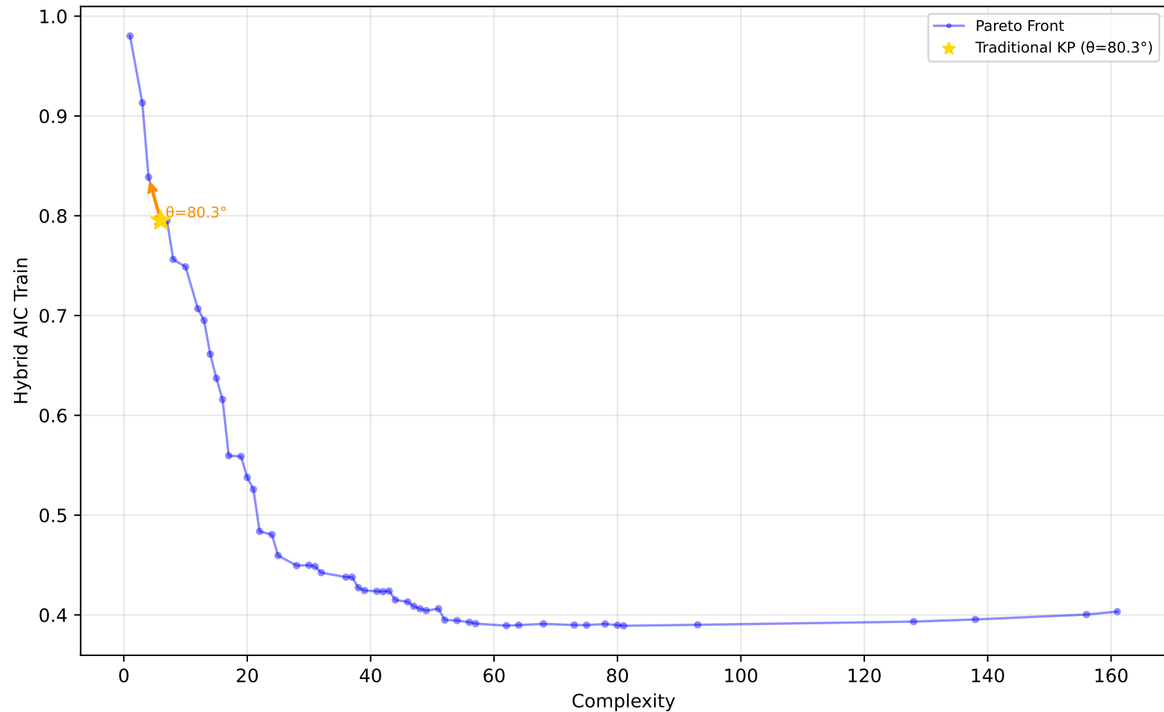
637_fri_c1_500_50 - Run 30 - MVP - Hybrid AIC Train \lambda_1=0.00, \lambda_2=0.50, \lambda_3=0.00 | Difficulty: 1.00 | Method: hmr
