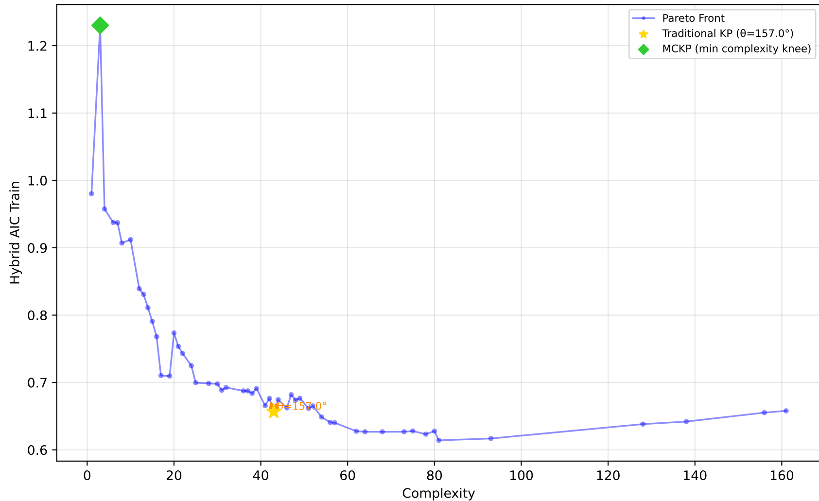
637_fri_c1_500_50 - Run 30 - MVP - Hybrid AIC Train \lambda_1=0.10, \lambda_2=0.00, \lambda_3=1.00 | Difficulty: 1.00 | Method: hmr
