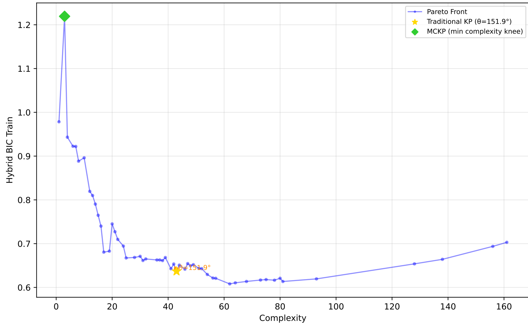
637_fri_c1_500_50 - Run 30 - MVP - Hybrid BIC Train \lambda_1=0.10, \lambda_2=0.00, \lambda_3=1.00 | Difficulty: 1.00 | Method: hmr
