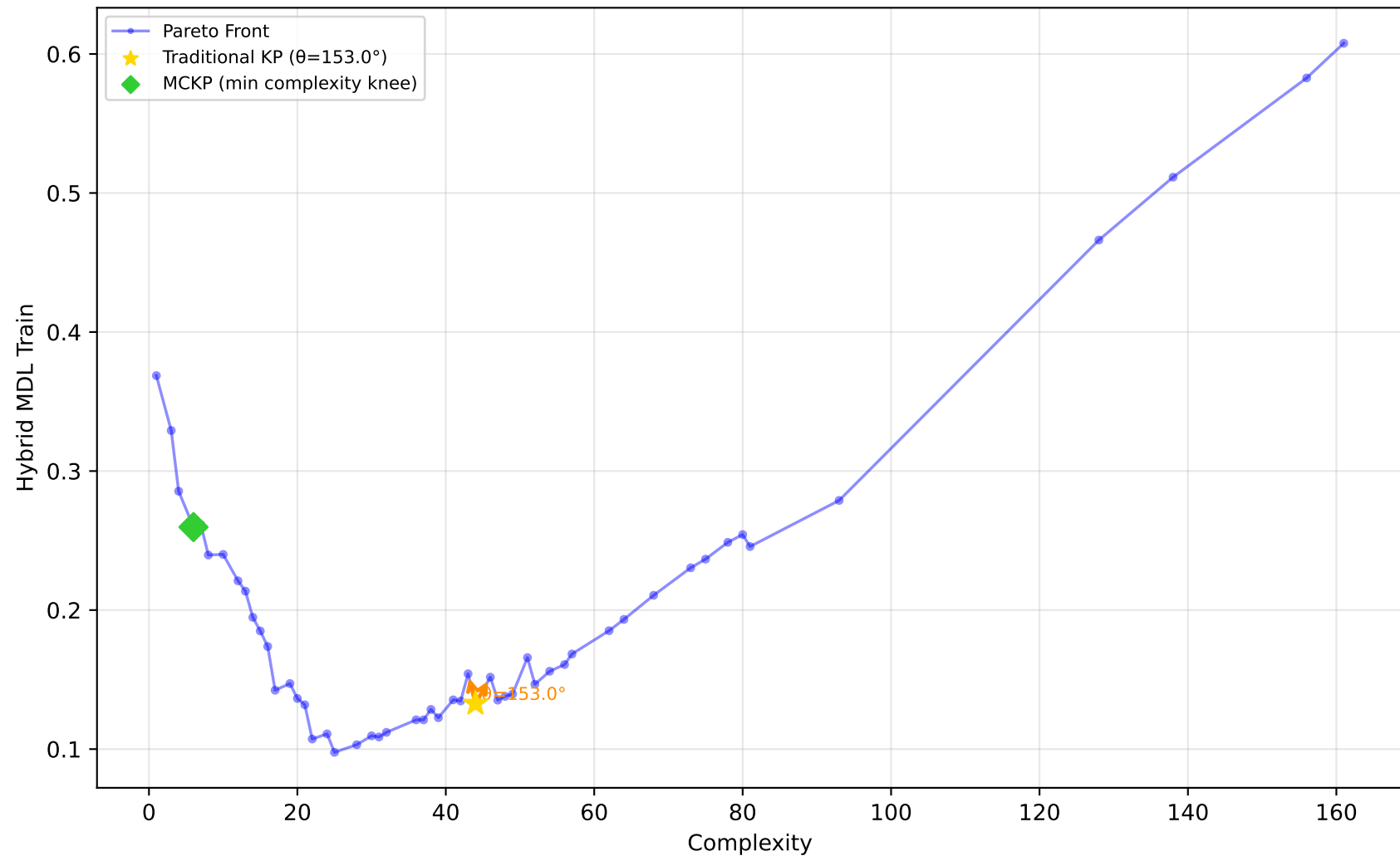
637_fri_c1_500_50 - Run 30 - MVP - Hybrid MDL Train \lambda_1=0.00, \lambda_2=0.50, \lambda_3=0.00 | Difficulty: 1.00 | Method: hmr
