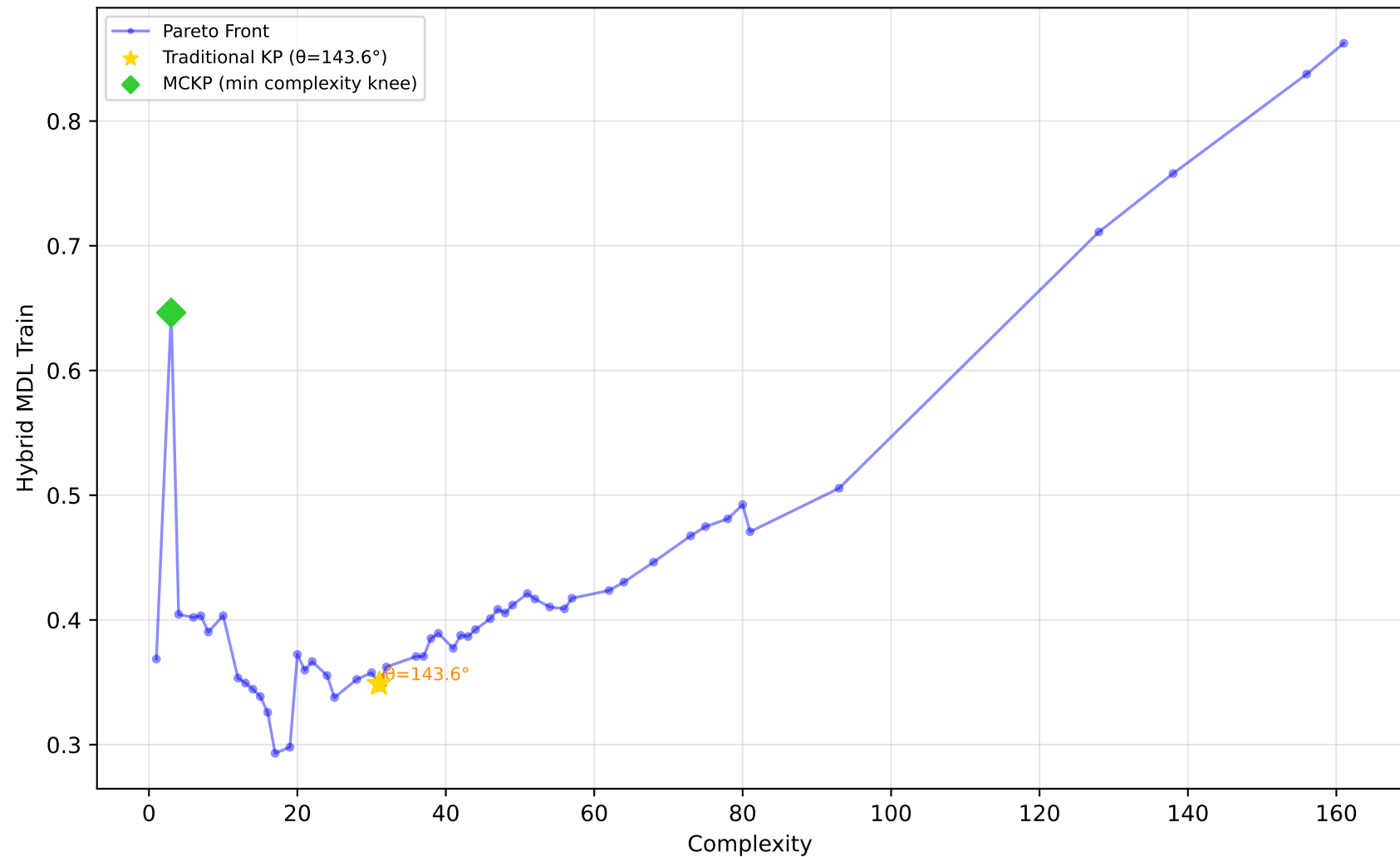
637_fri_c1_500_50 - Run 30 - MVP - Hybrid MDL Train \lambda_1=0.10, \bar{\lambda}_2=0.00, \lambda_3=1.00 | Difficulty: 1.00 | Method: hmr
