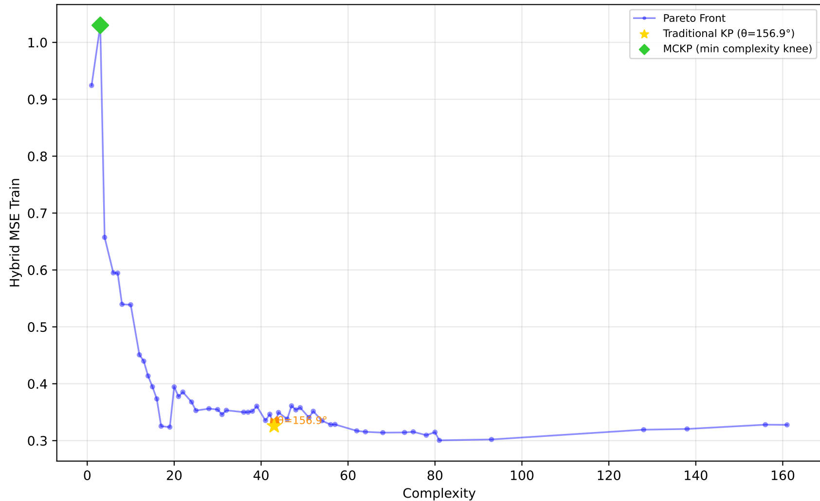
637_fri_c1_500_50 - Run 30 - MVP - Hybrid MSE Train \lambda_1=0.10, \bar{\lambda}_2=0.00, \lambda_3=1.00 | Difficulty: 1.00 | Method: hmr
