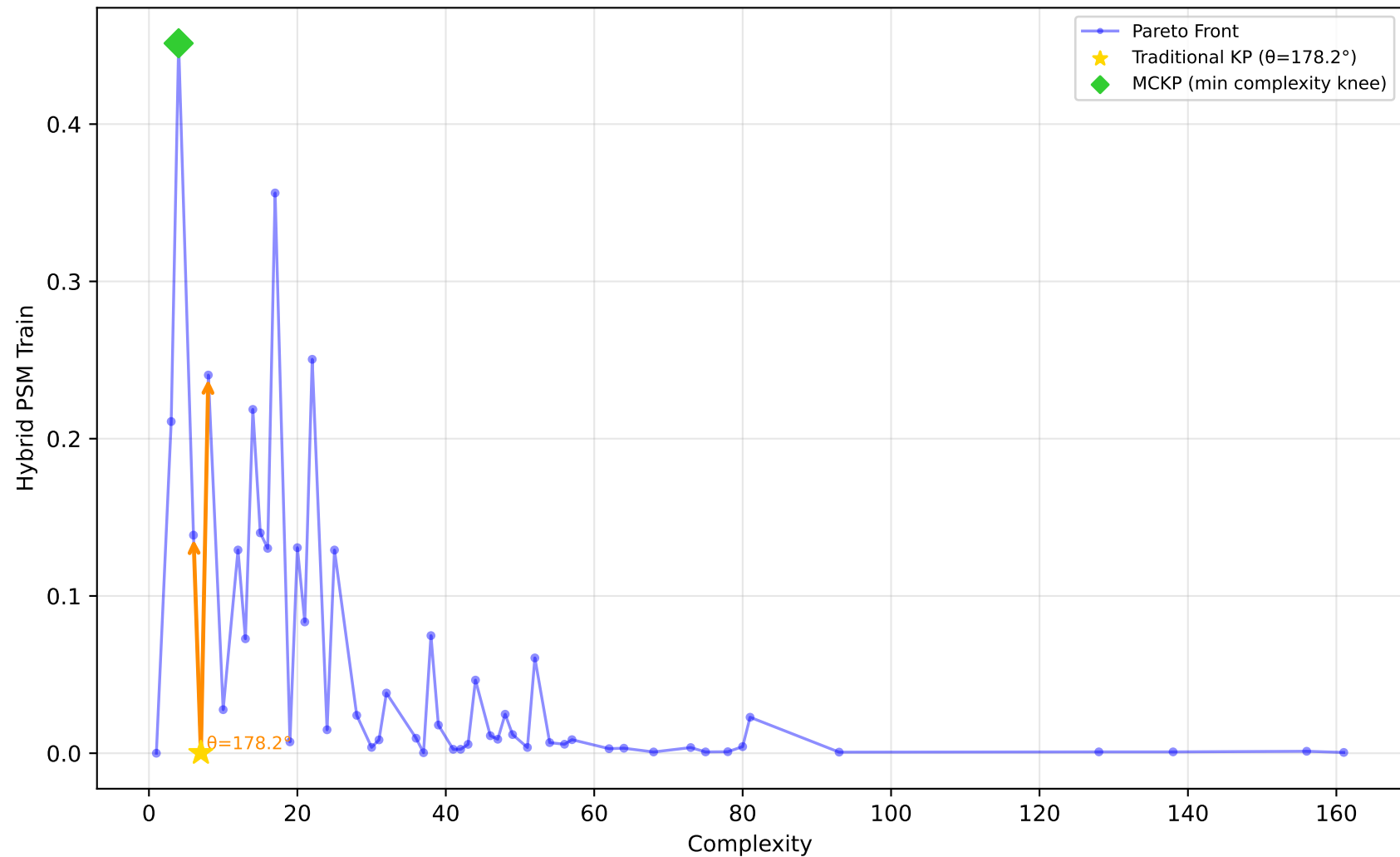
637_fri_c1_500_50 - Run 30 - MVP - Hybrid PSM Train \lambda_1=0.00, \bar{\lambda}_2=0.50, \lambda_3=0.00 | Difficulty: 1.00 | Method: hmr
