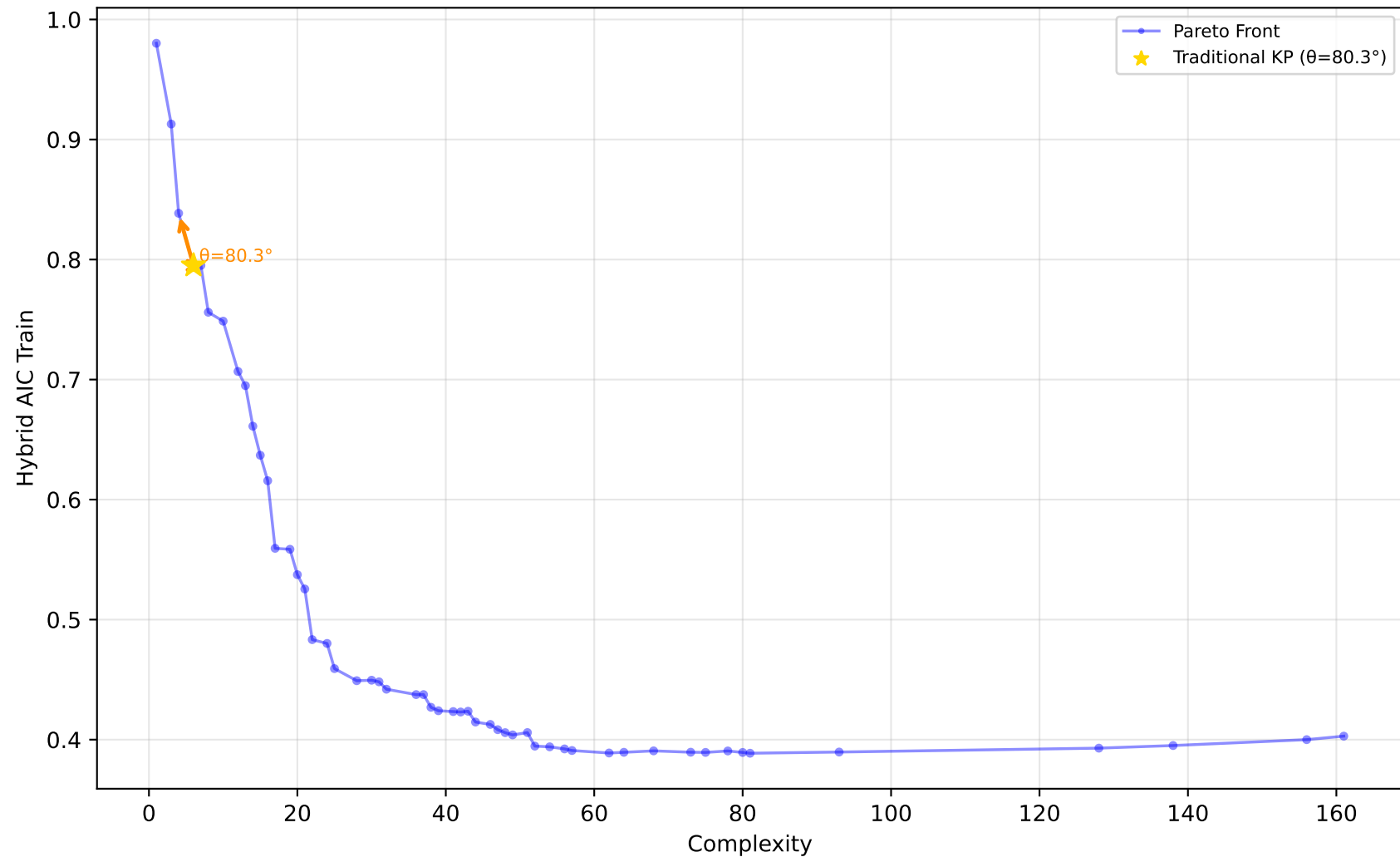
637_fri_c1_500_50 - Run 30 - SVP - Hybrid AIC Train \lambda_1=0.00, \lambda_2=0.00, \lambda_3=0.00 | Difficulty: 1.00 | Method: hmr
