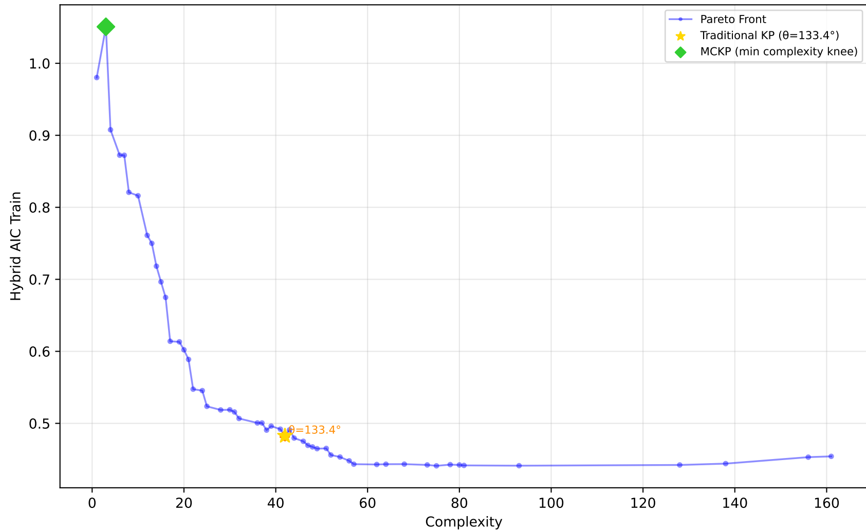
637_fri_c1_500_50 - Run 30 - SVP - Hybrid AIC Train \lambda_1=0.10, \lambda_2=0.00, \lambda_3=0.20 | Difficulty: 1.00 | Method: hmr
