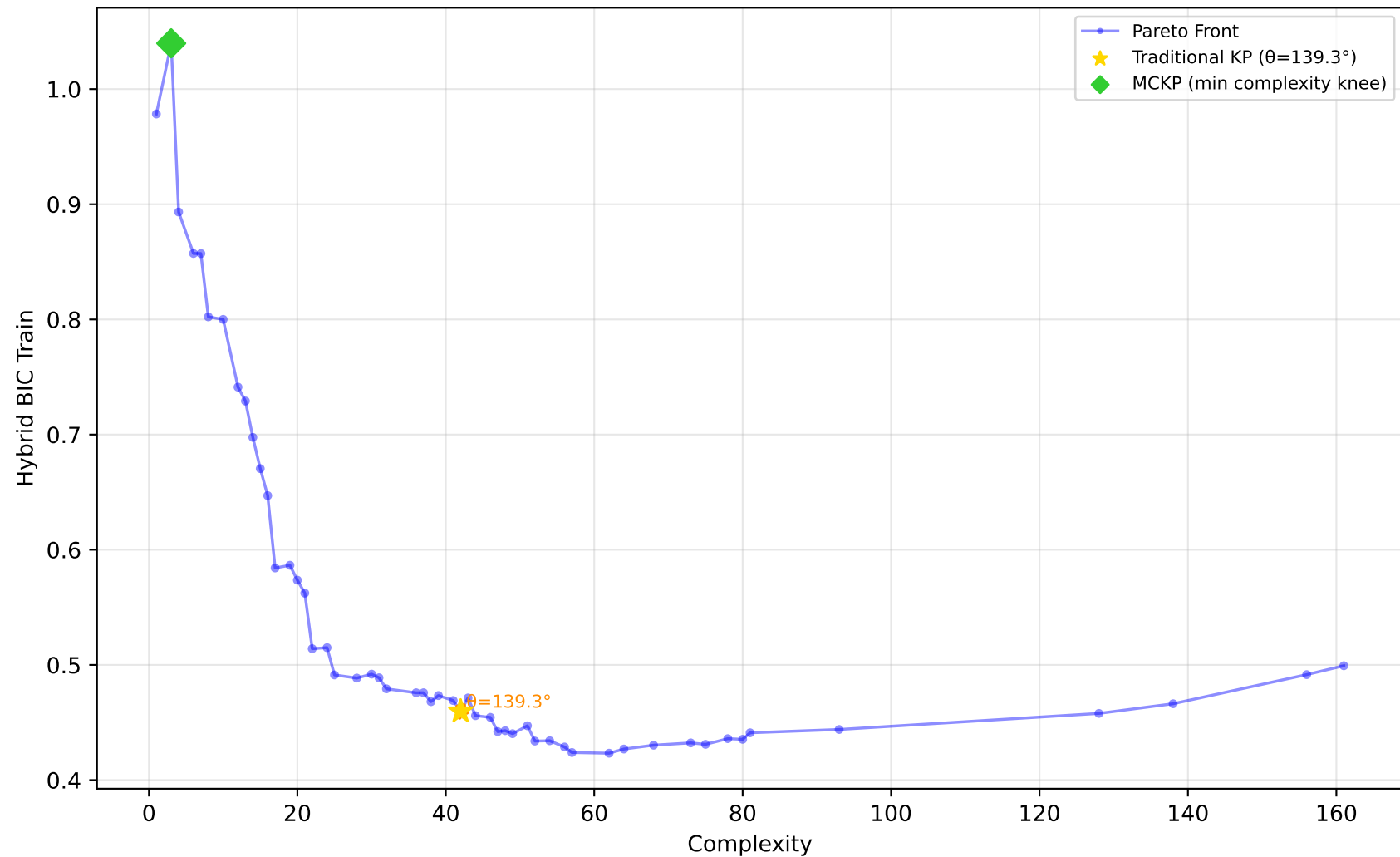
637_fri_c1_500_50 - Run 30 - SVP - Hybrid BIC Train \lambda_1=0.10, \lambda_2=0.00, \lambda_3=0.20 | Difficulty: 1.00 | Method: hmr
