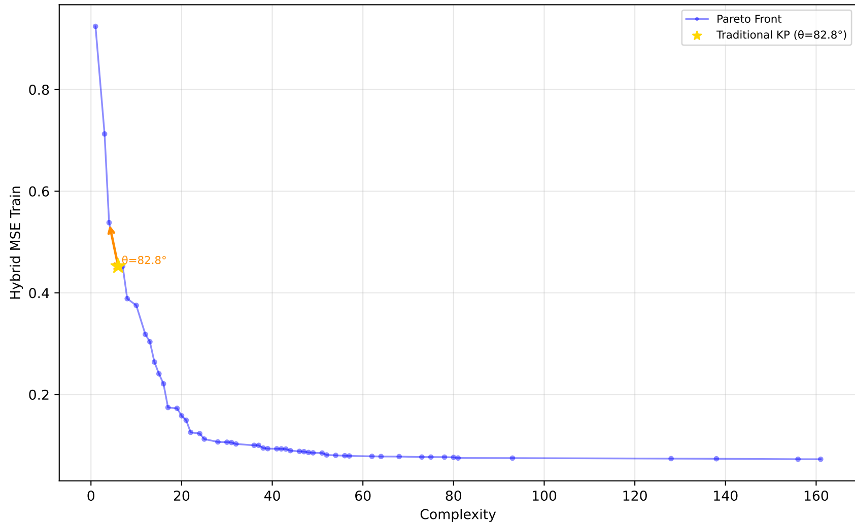
637_fri_c1_500_50 - Run 30 - SVP - Hybrid MSE Train \lambda_1=0.00, \lambda_2=0.00, \lambda_3=0.00 | Difficulty: 1.00 | Method: hmr
