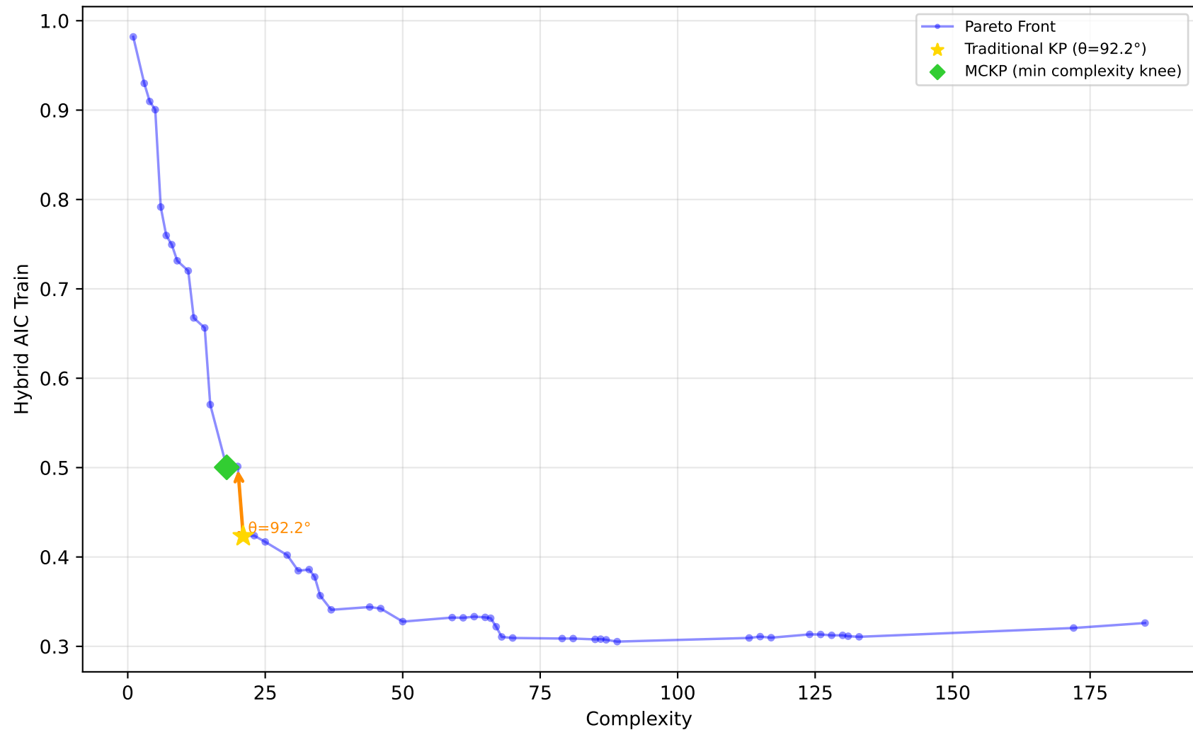
637_fri_c1_500_50 - Run 3 - MVP - Hybrid AIC Train \lambda_1=0.00, \lambda_2=0.50, \lambda_3=0.00 | Difficulty: 1.00 | Method: hmr
