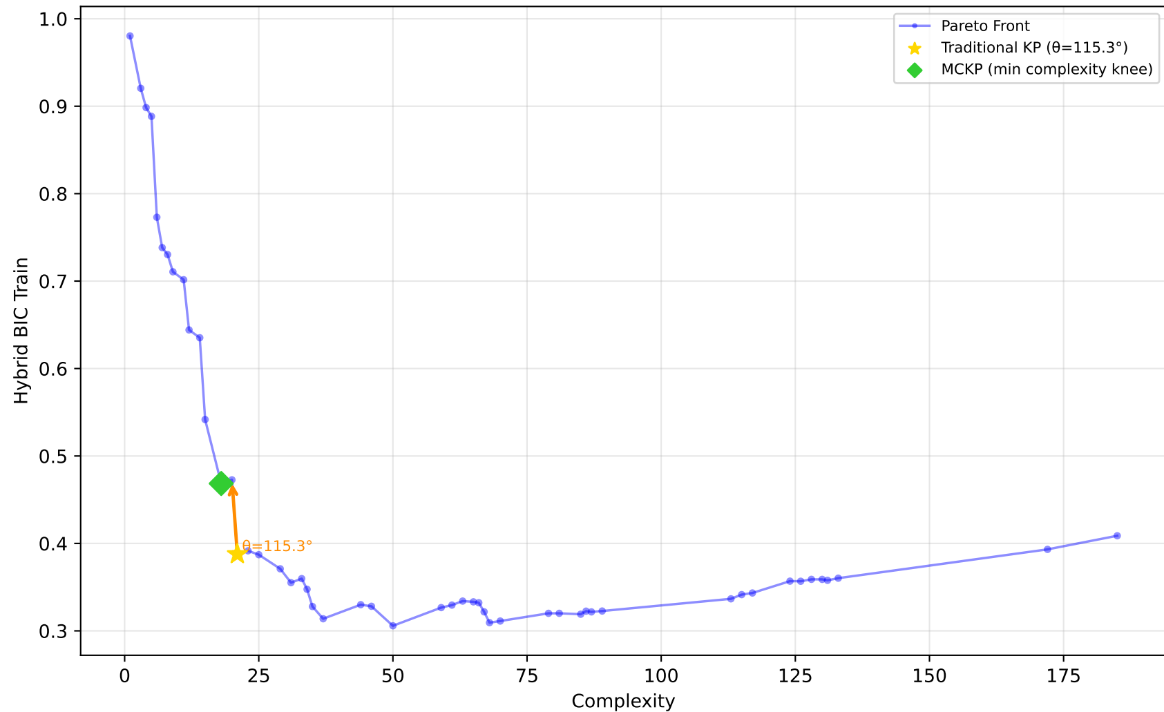
637_fri_c1_500_50 - Run 3 - MVP - Hybrid BIC Train \lambda_1=0.00, \lambda_2=0.50, \lambda_3=0.00 | Difficulty: 1.00 | Method: hmr
