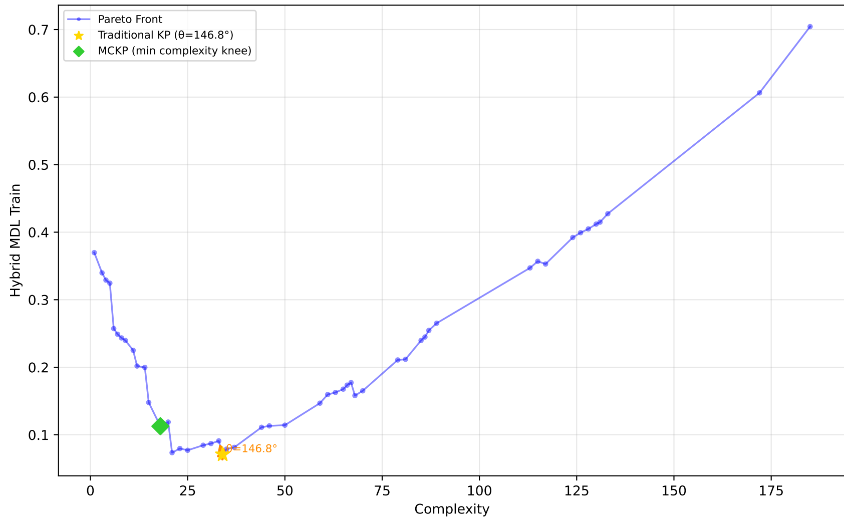
637_fri_c1_500_50 - Run 3 - MVP - Hybrid MDL Train \lambda_1=0.00, \lambda_2=0.50, \lambda_3=0.00 | Difficulty: 1.00 | Method: hmr
