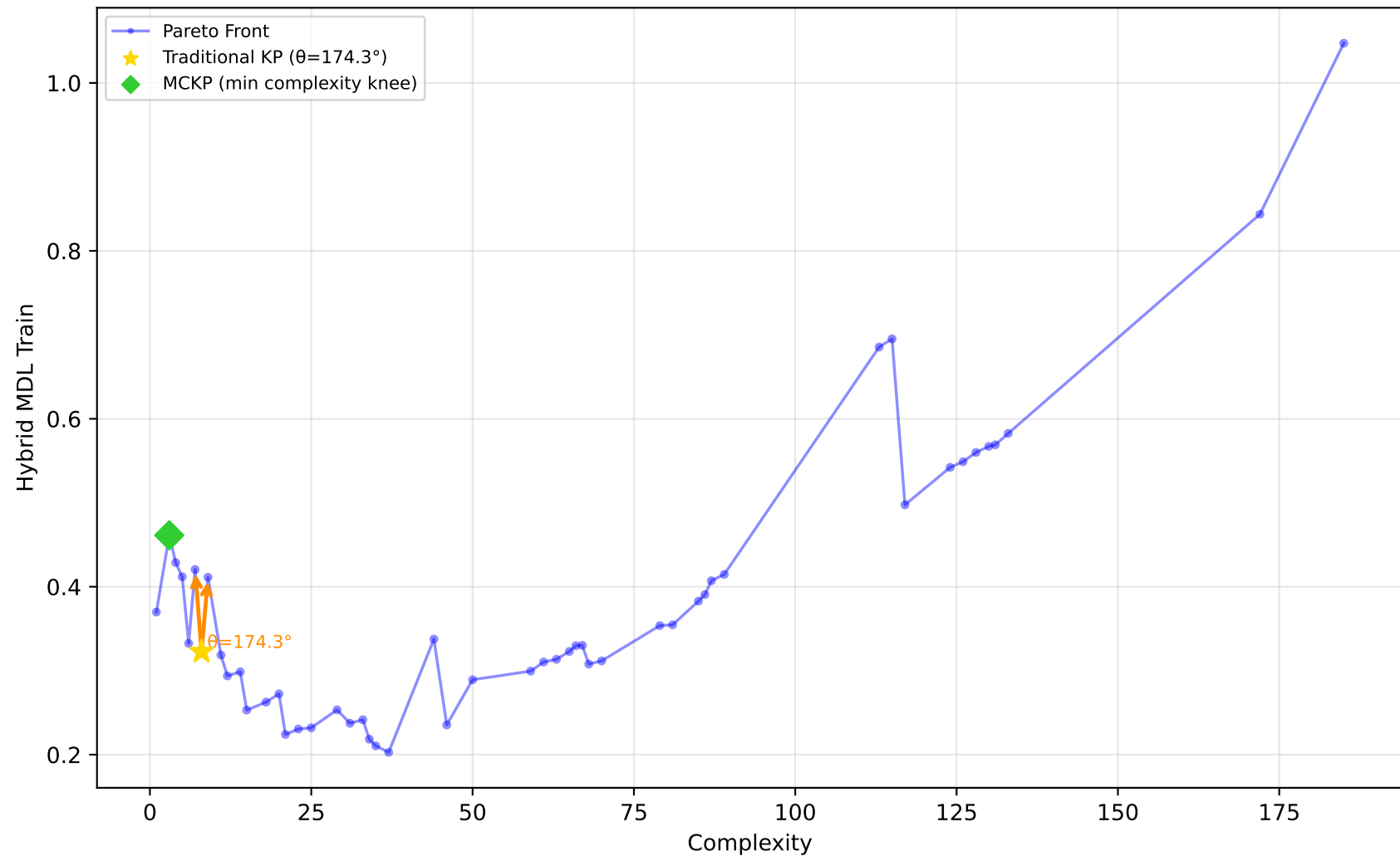
637_fri_c1_500_50 - Run 3 - MVP - Hybrid MDL Train \lambda_1=0.10, \lambda_2=0.00, \lambda_3=1.00 | Difficulty: 1.00 | Method: hmr
