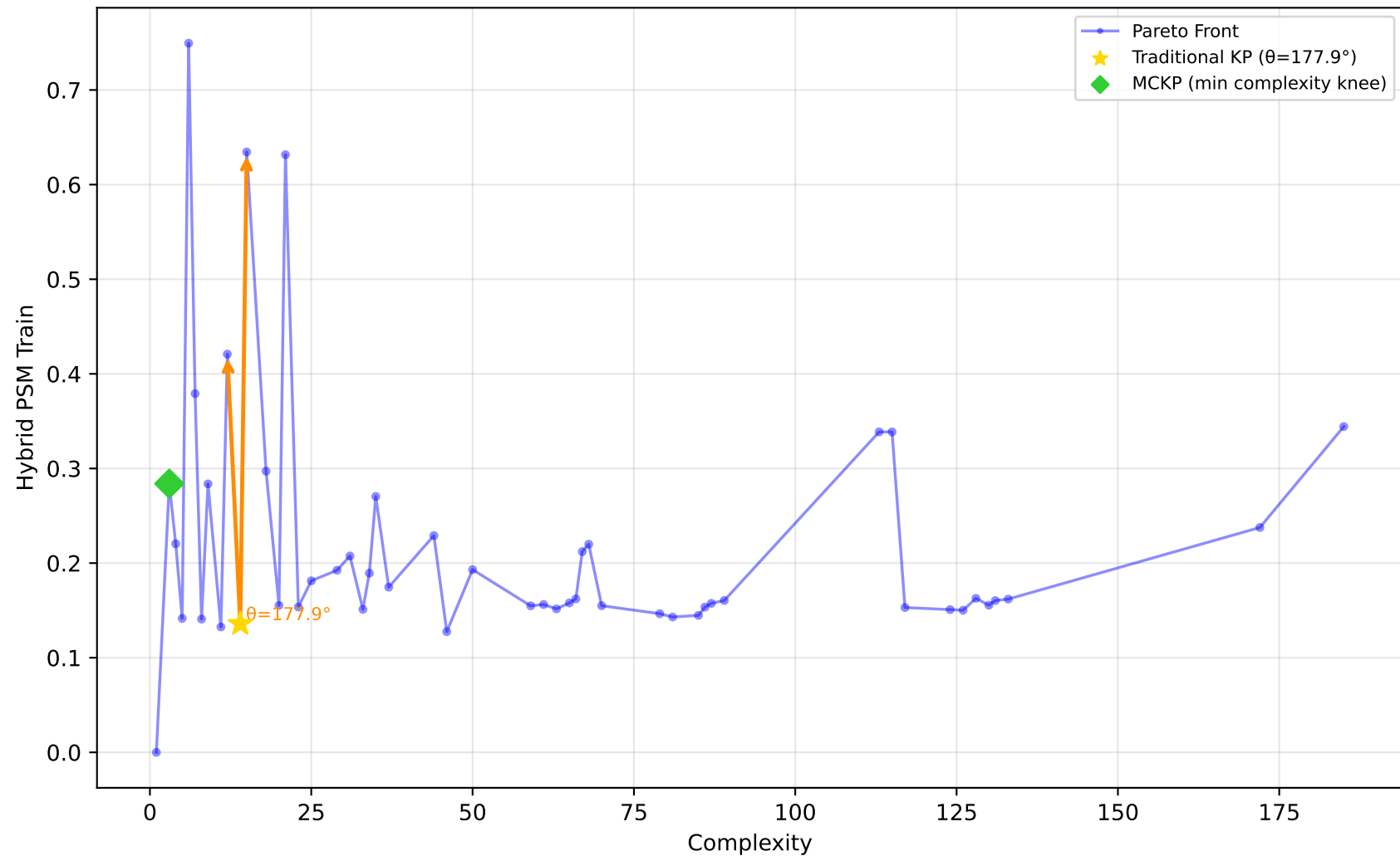
637_fri_c1_500_50 - Run 3 - MVP - Hybrid PSM Train \lambda_1=0.10, \lambda_2=0.00, \lambda_3=1.00 | Difficulty: 1.00 | Method: hmr
