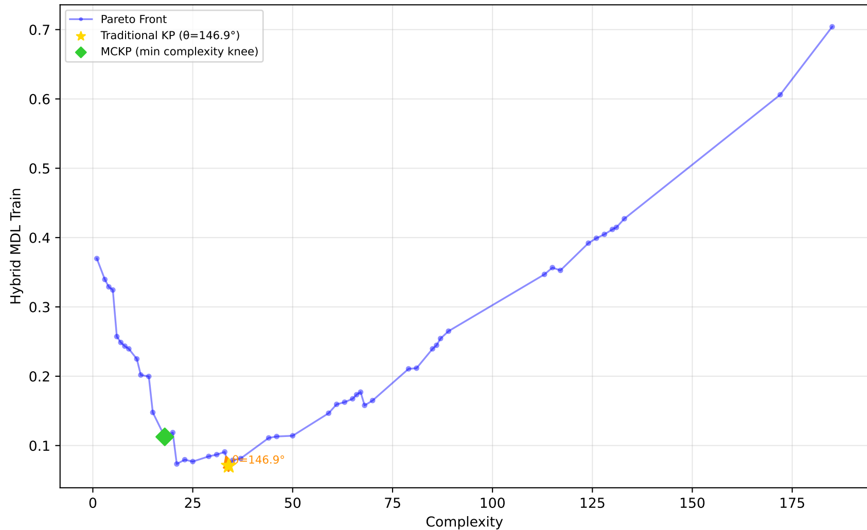
637_fri_c1_500_50 - Run 3 - SVP - Hybrid MDL Train \lambda_1=0.00, \lambda_2=0.00, \lambda_3=0.00 | Difficulty: 1.00 | Method: hmr
