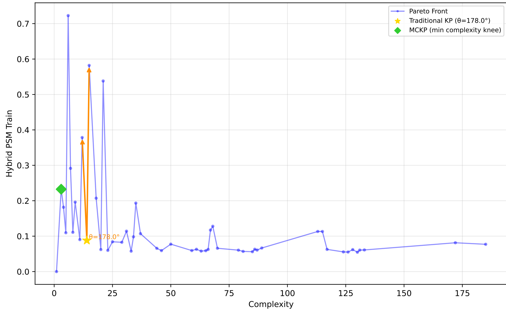
637_fri_c1_500_50 - Run 3 - SVP - Hybrid PSM Train \lambda_1=0.10, \lambda_2=0.00, \lambda_3=0.20 | Difficulty: 1.00 | Method: hmr
