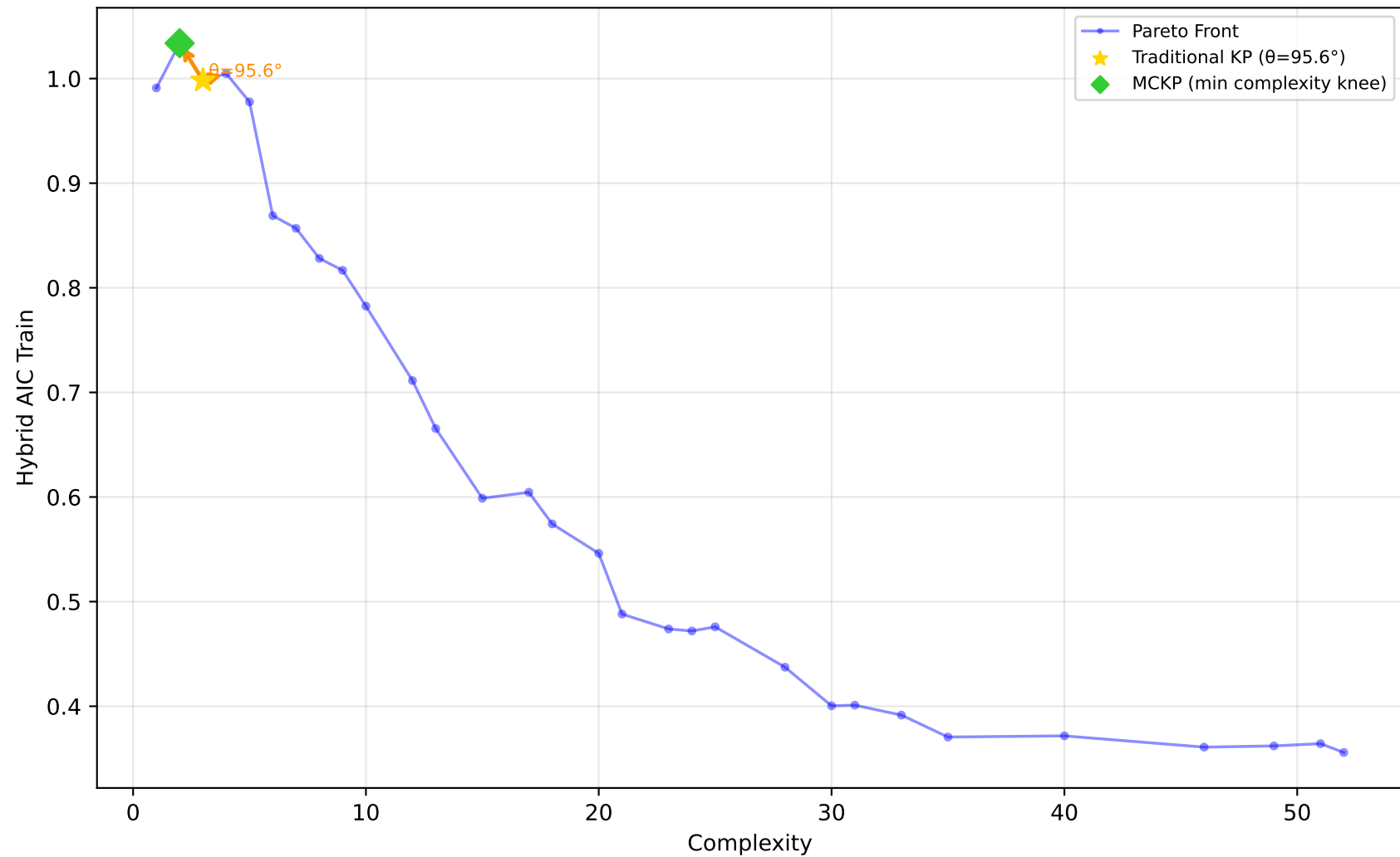
637_fri_c1_500_50 - Run 4 - MVP - Hybrid AIC Train \lambda_1=0.10 , \lambda_2=0.00 , \lambda_3=1.00 | Difficulty: 1.00 | Method: hmr
