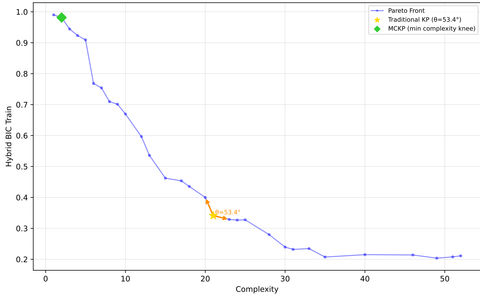
637_fri_c1_500_50 - Run 4 - MVP - Hybrid BIC Train \lambda_1=0.00, \lambda_2=0.50, \lambda_3=0.00 | Difficulty: 1.00 | Method: hmr
