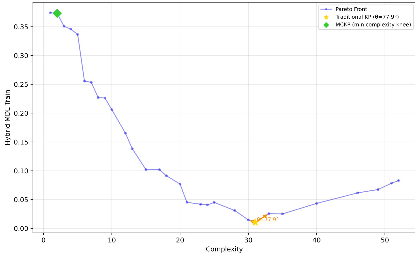
637_fri_c1_500_50 - Run 4 - MVP - Hybrid MDL Train \lambda_1=0.00, \lambda_2=0.50, \lambda_3=0.00 | Difficulty: 1.00 | Method: hmr
