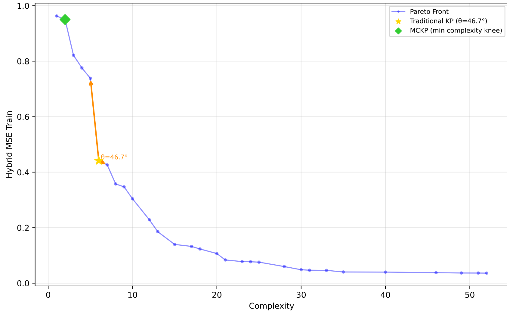
637_fri_c1_500_50 - Run 4 - MVP - Hybrid MSE Train \lambda_1=0.00, \lambda_2=0.50, \lambda_3=0.00 | Difficulty: 1.00 | Method: hmr
