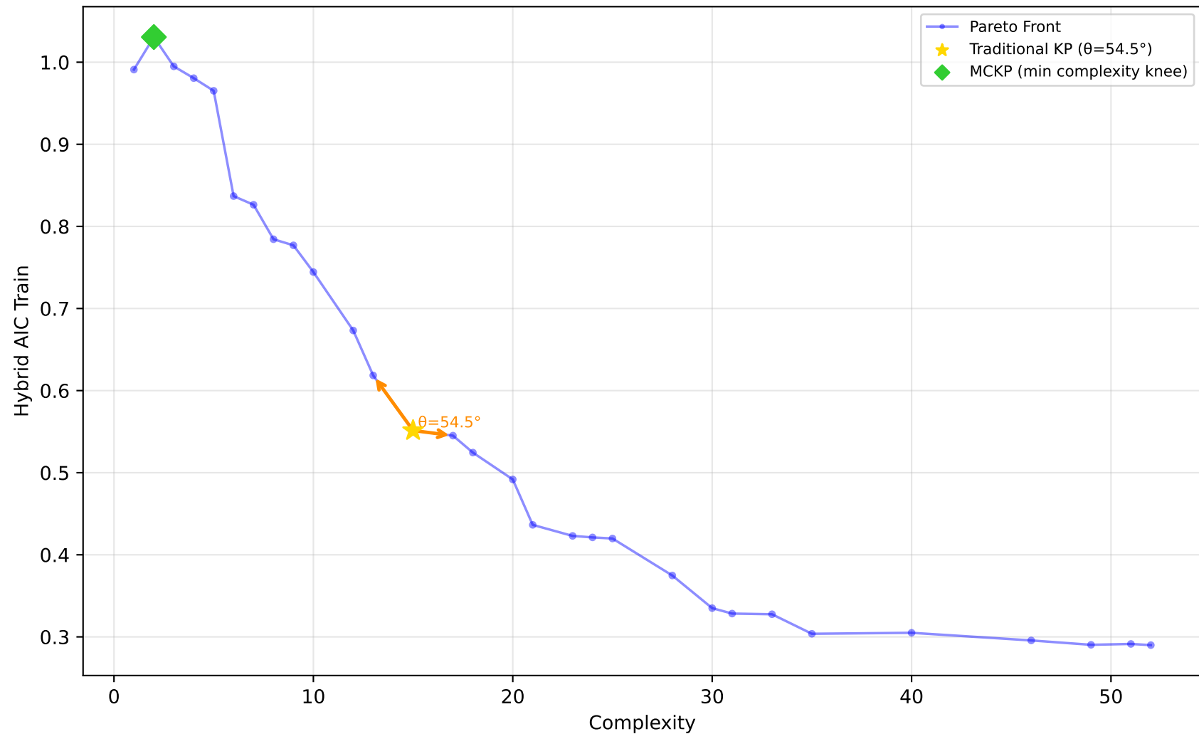
637_fri_c1_500_50 - Run 4 - SVP - Hybrid AIC Train \lambda_1=0.10, \lambda_2=0.00, \lambda_3=0.20 | Difficulty: 1.00 | Method: hmr
