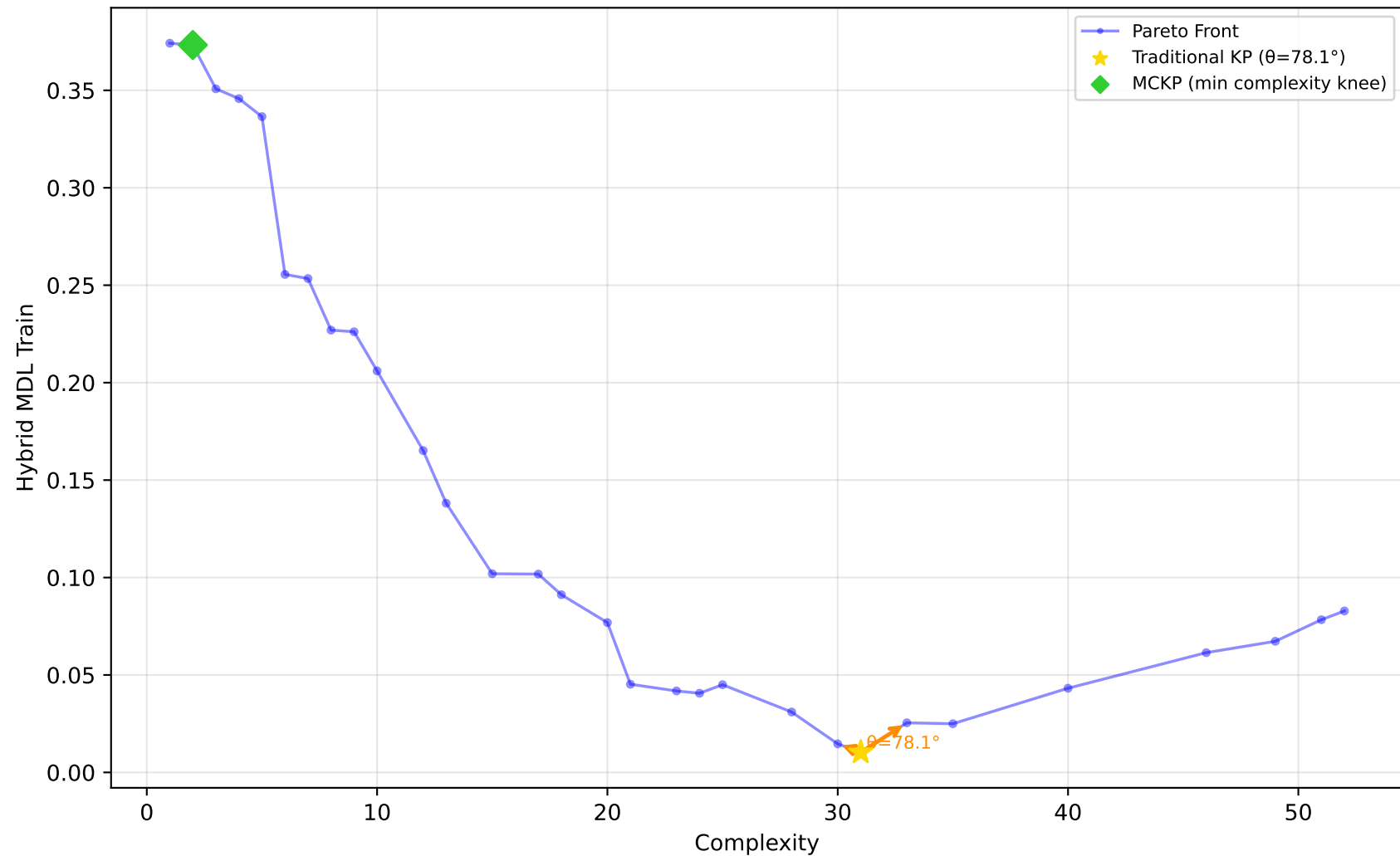
637_fri_c1_500_50 - Run 4 - SVP - Hybrid MDL Train \lambda_1=0.00, \lambda_2=0.00, \bar{\lambda}_3=0.00 | Difficulty: 1.00 | Method: hmr
