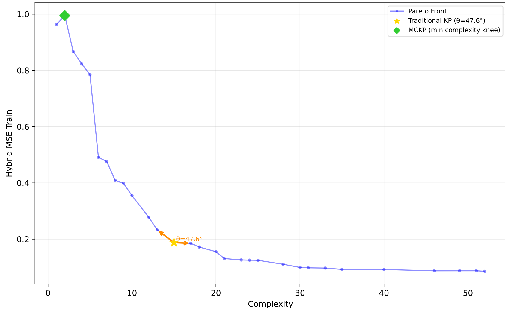
637_fri_c1_500_50 - Run 4 - SVP - Hybrid MSE Train \lambda_1=0.10, \lambda_2=0.00, \lambda_3=0.20 | Difficulty: 1.00 | Method: hmr
