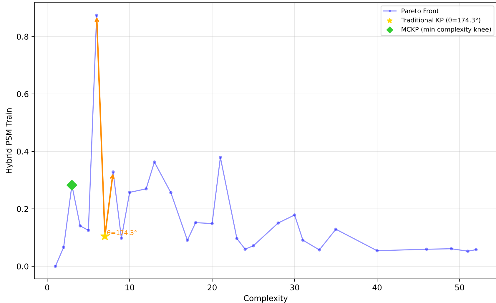
637_fri_c1_500_50 - Run 4 - SVP - Hybrid PSM Train \lambda_1=0.10, \lambda_2=0.00, \lambda_3=0.20 | Difficulty: 1.00 | Method: hmr
