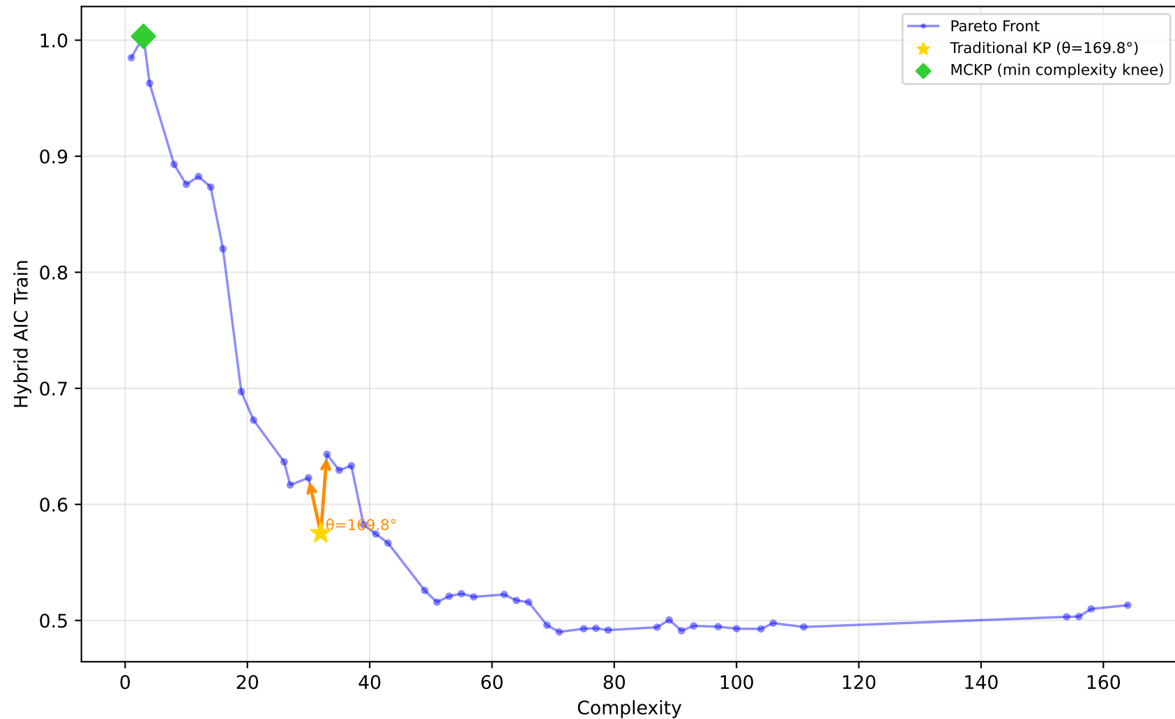
637_fri_c1_500_50 - Run 5 - MVP - Hybrid AIC Train \lambda_1=0.10, \lambda_2=0.00, \lambda_3=1.00 | Difficulty: 1.00 | Method: hmr
