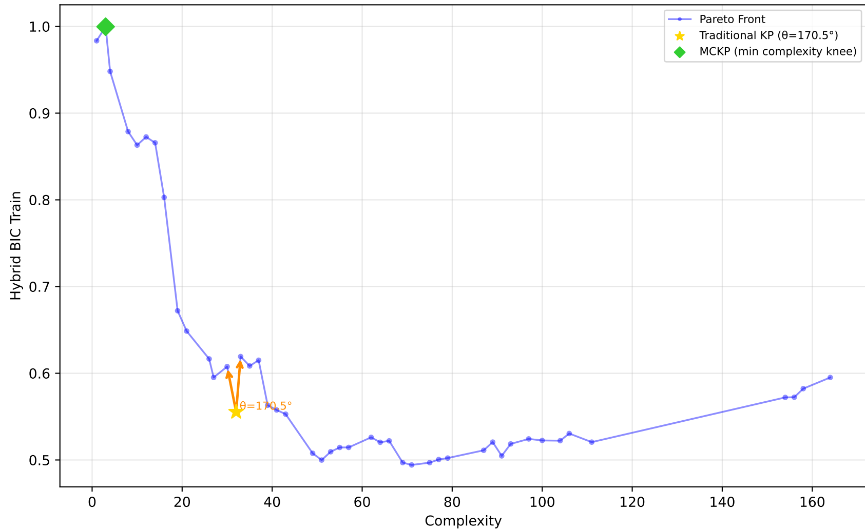
637_fri_c1_500_50 - Run 5 - MVP - Hybrid BIC Train \lambda_1=0.10, \lambda_2=0.00, \lambda_3=1.00 | Difficulty: 1.00 | Method: hmr
