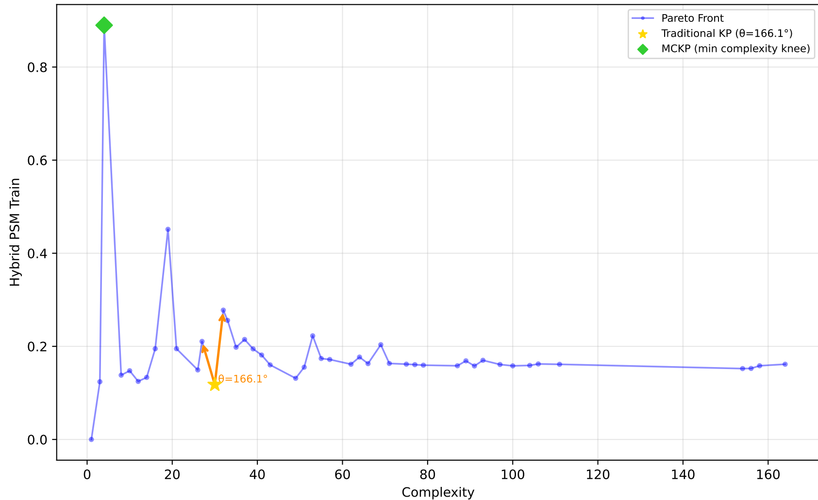
637_fri_c1_500_50 - Run 5 - MVP - Hybrid PSM Train \lambda_1=0.10, \lambda_2=0.00, \lambda_3=1.00 | Difficulty: 1.00 | Method: hmr
