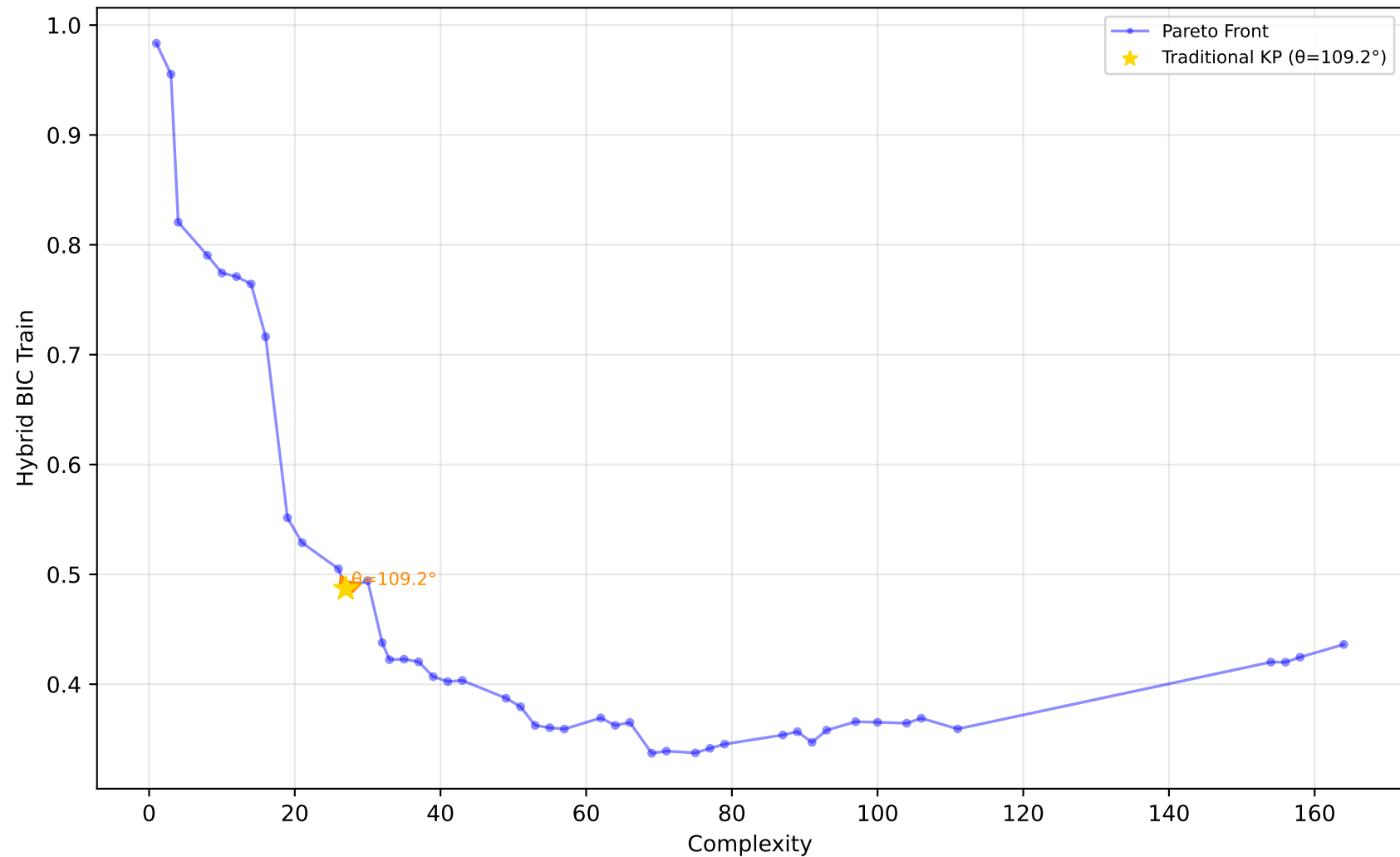
637_fri_c1_500_50 - Run 5 - SVP - Hybrid BIC Train \lambda_1=0.00, \lambda_2=0.00, \lambda_3=0.00 | Difficulty: 1.00 | Method: hmr
