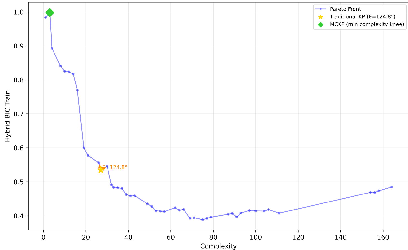
637_fri_c1_500_50 - Run 5 - SVP - Hybrid BIC Train \lambda_1=0.10, \lambda_2=0.00, \lambda_3=0.20 | Difficulty: 1.00 | Method: hmr
