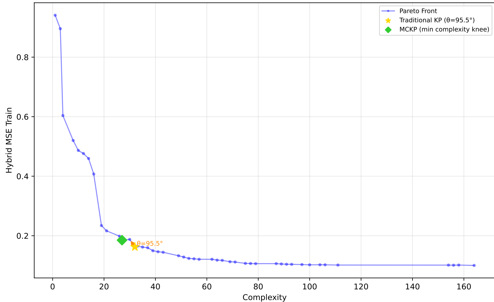
637_fri_c1_500_50 - Run 5 - SVP - Hybrid MSE Train \lambda_1=0.10, \lambda_2=0.00, \lambda_3=0.20 | Difficulty: 1.00 | Method: hmr
