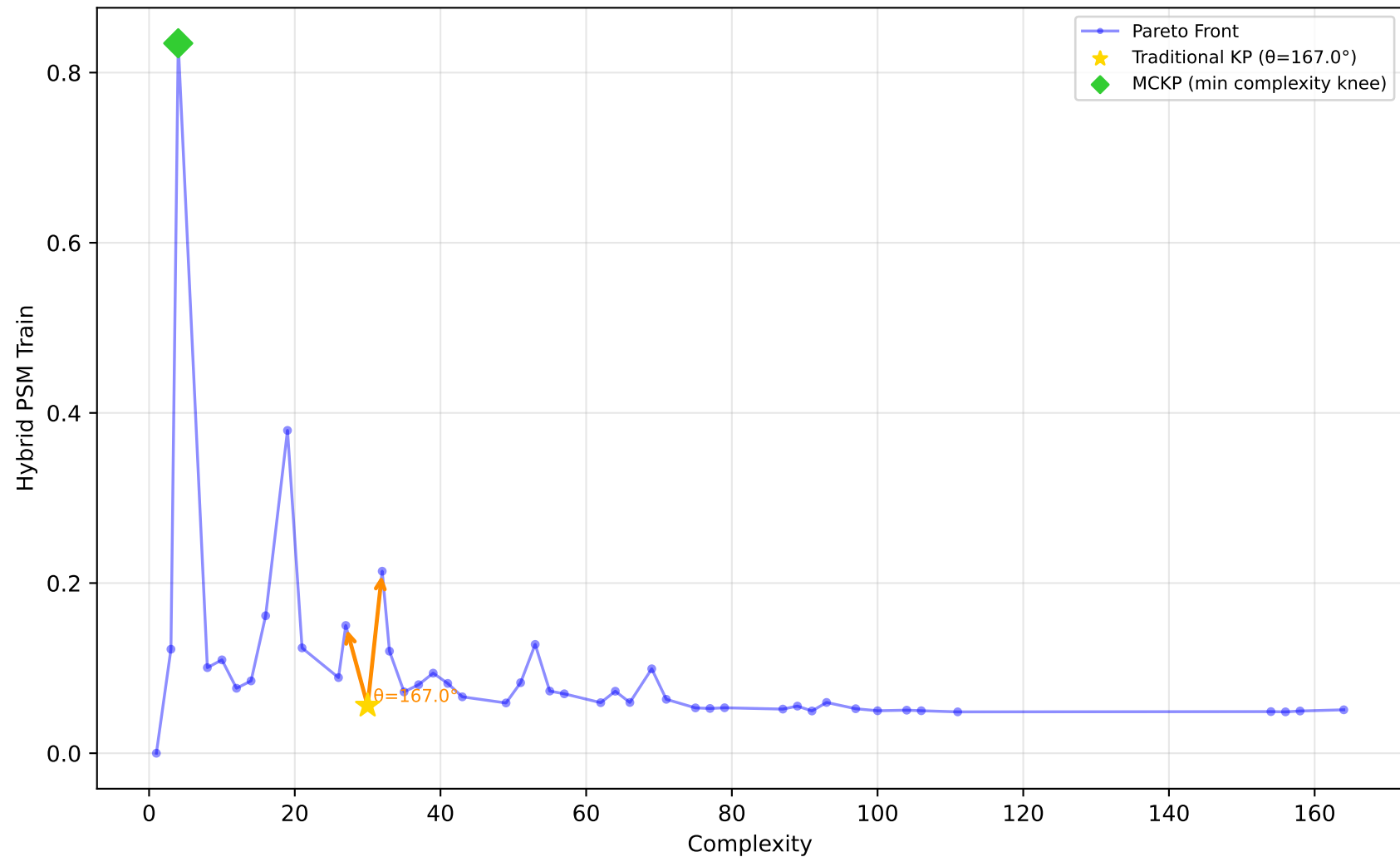
637_fri_c1_500_50 - Run 5 - SVP - Hybrid PSM Train \lambda_1=0.10, \lambda_2=0.00, \lambda_3=0.20 | Difficulty: 1.00 | Method: hmr
