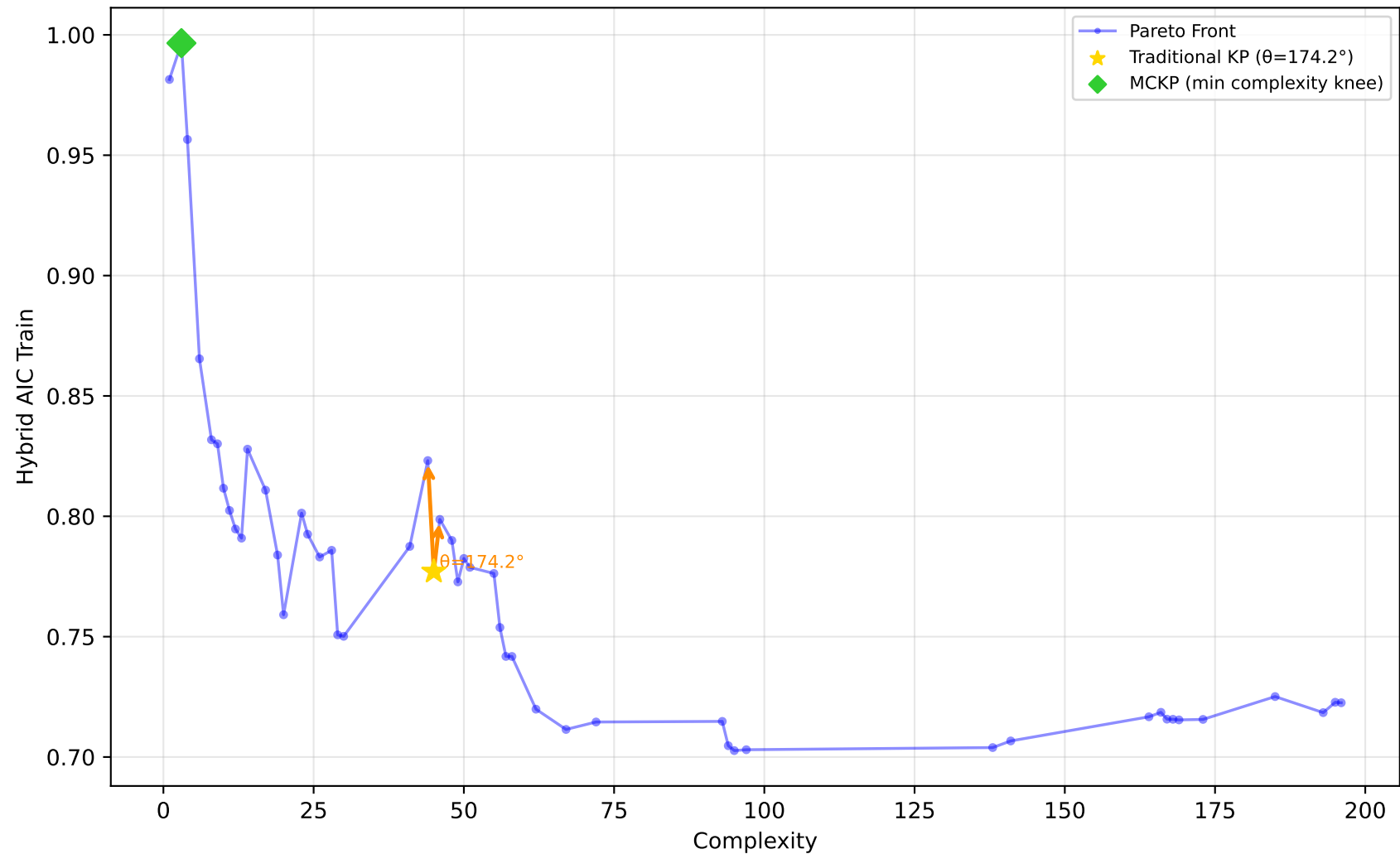
637_fri_c1_500_50 - Run 6 - MVP - Hybrid AIC Train \lambda_1=0.10, \lambda_2=0.00, \bar{\lambda}_3=1.00 | Difficulty: 1.00 | Method: hmr
