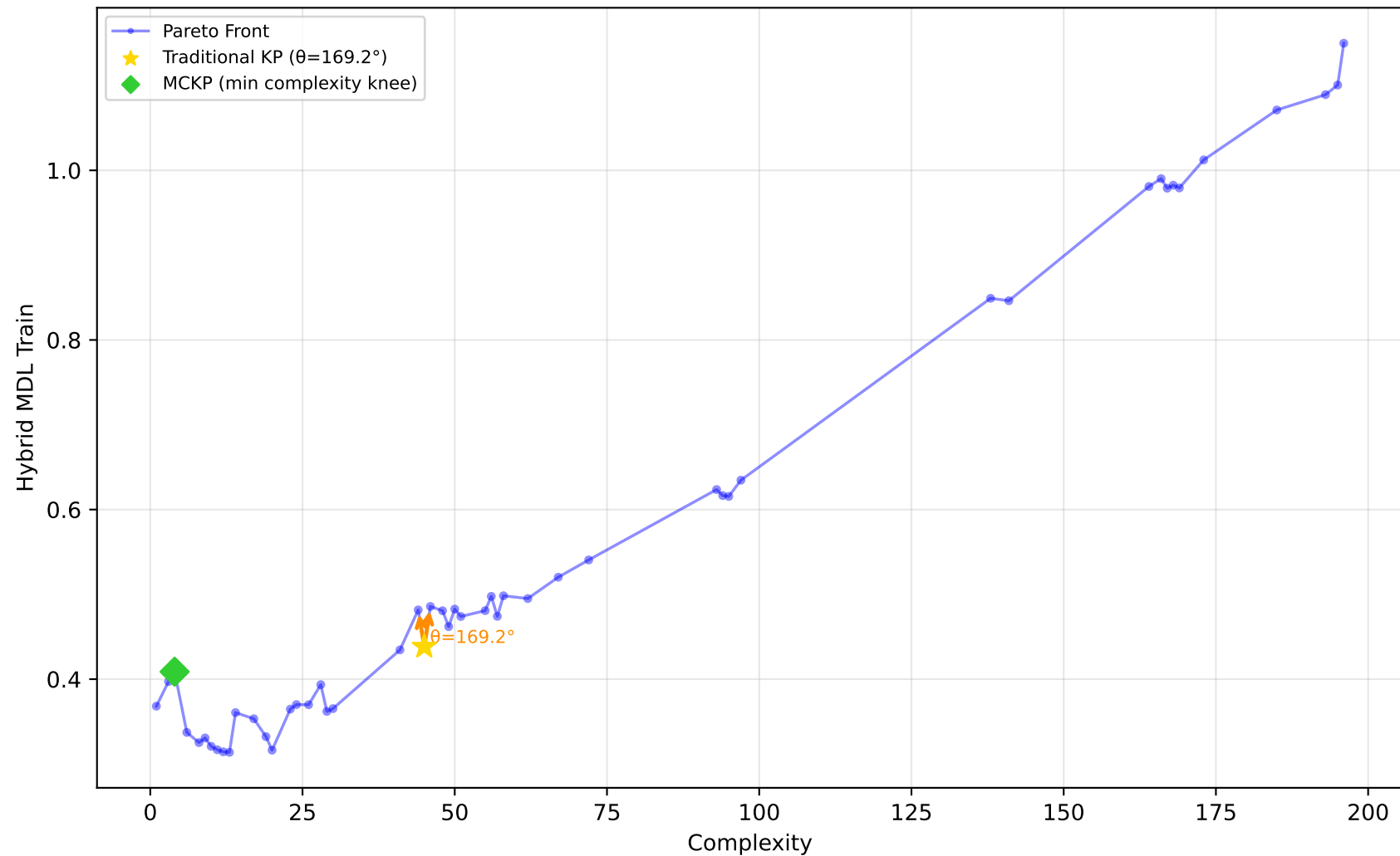
637_fri_c1_500_50 - Run 6 - MVP - Hybrid MDL Train \lambda_1=0.10, \lambda_2=0.00, \lambda_3=1.00 | Difficulty: 1.00 | Method: hmr
