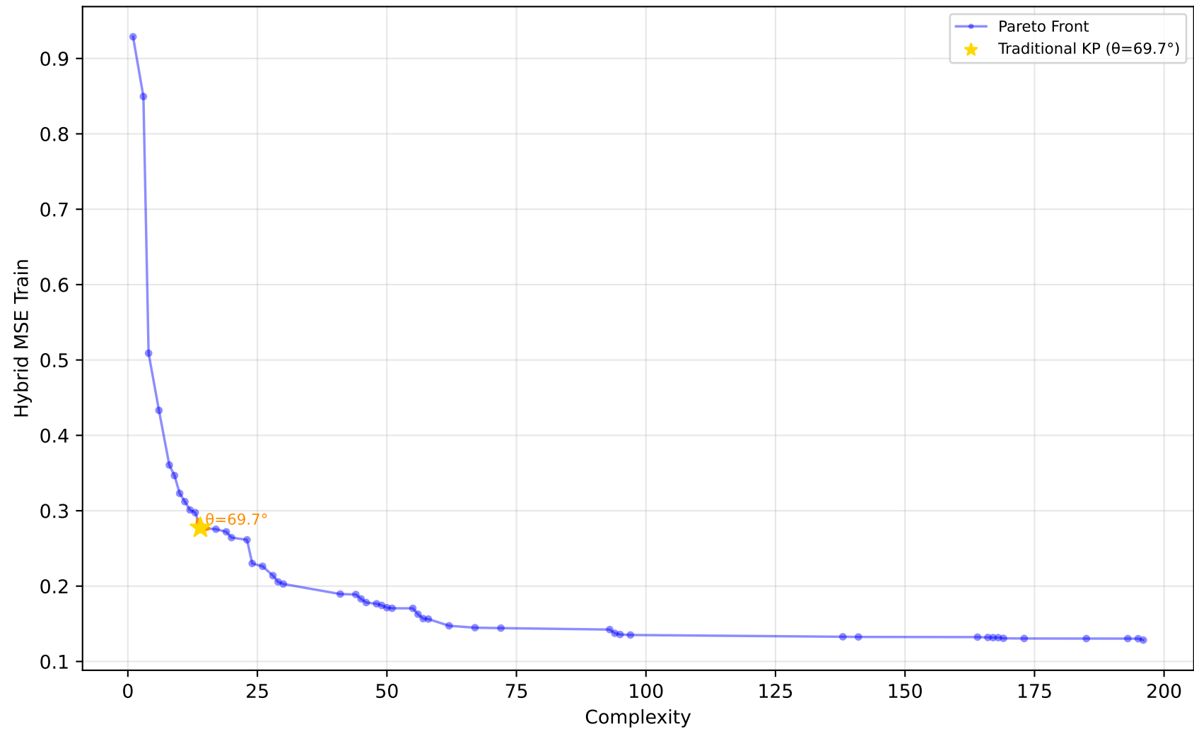
637_fri_c1_500_50 - Run 6 - MVP - Hybrid MSE Train \lambda_1=0.00, \lambda_2=0.50, \lambda_3=0.00 | Difficulty: 1.00 | Method: hmr
