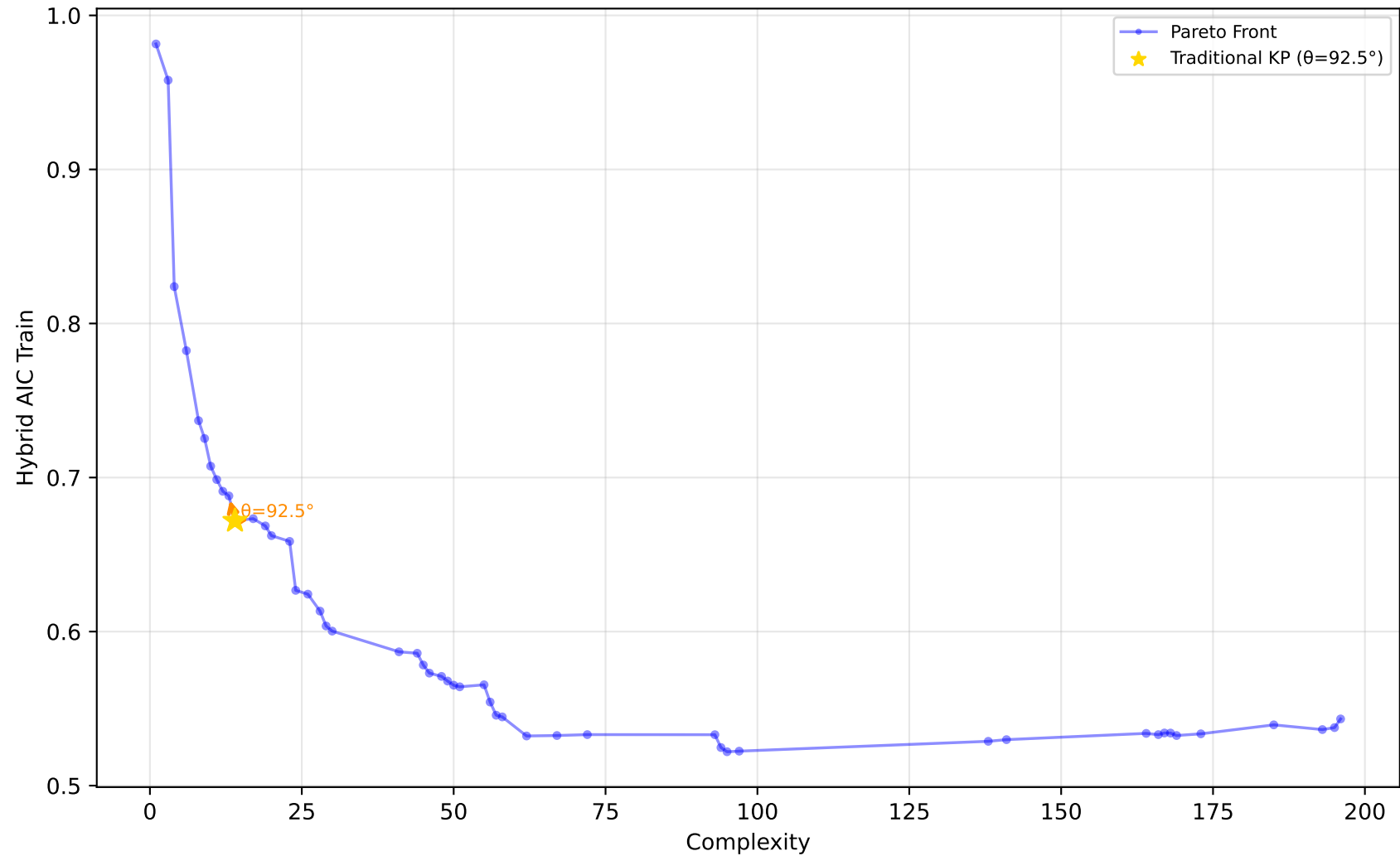
637_fri_c1_500_50 - Run 6 - SVP - Hybrid AIC Train \lambda_1=0.00, \lambda_2=0.00, \lambda_3=0.00 | Difficulty: 1.00 | Method: hmr
