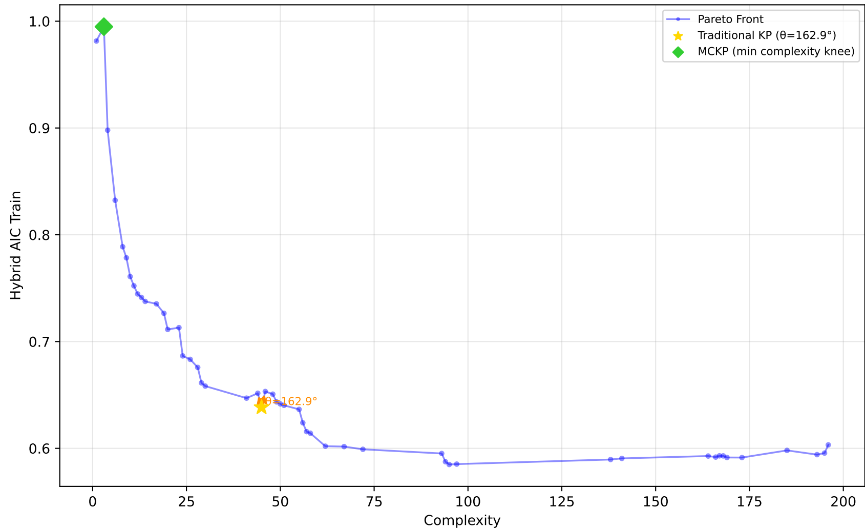
637_fri_c1_500_50 - Run 6 - SVP - Hybrid AIC Train \lambda_1=0.10, \lambda_2=0.00, \lambda_3=0.20 | Difficulty: 1.00 | Method: hmr
