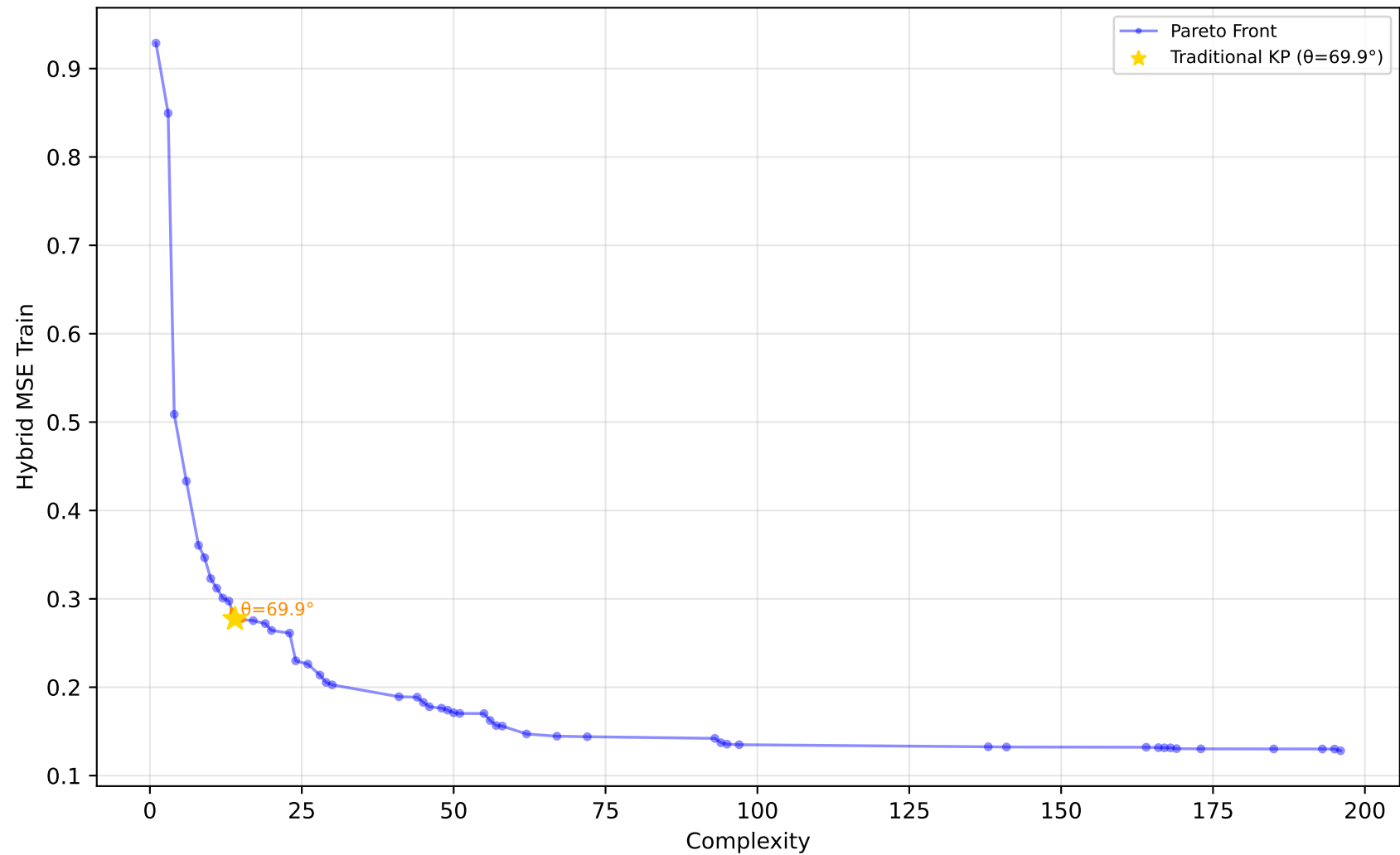
637_fri_c1_500_50 - Run 6 - SVP - Hybrid MSE Train \lambda_1=0.00, \lambda_2=0.00, \lambda_3=0.00 | Difficulty: 1.00 | Method: hmr
