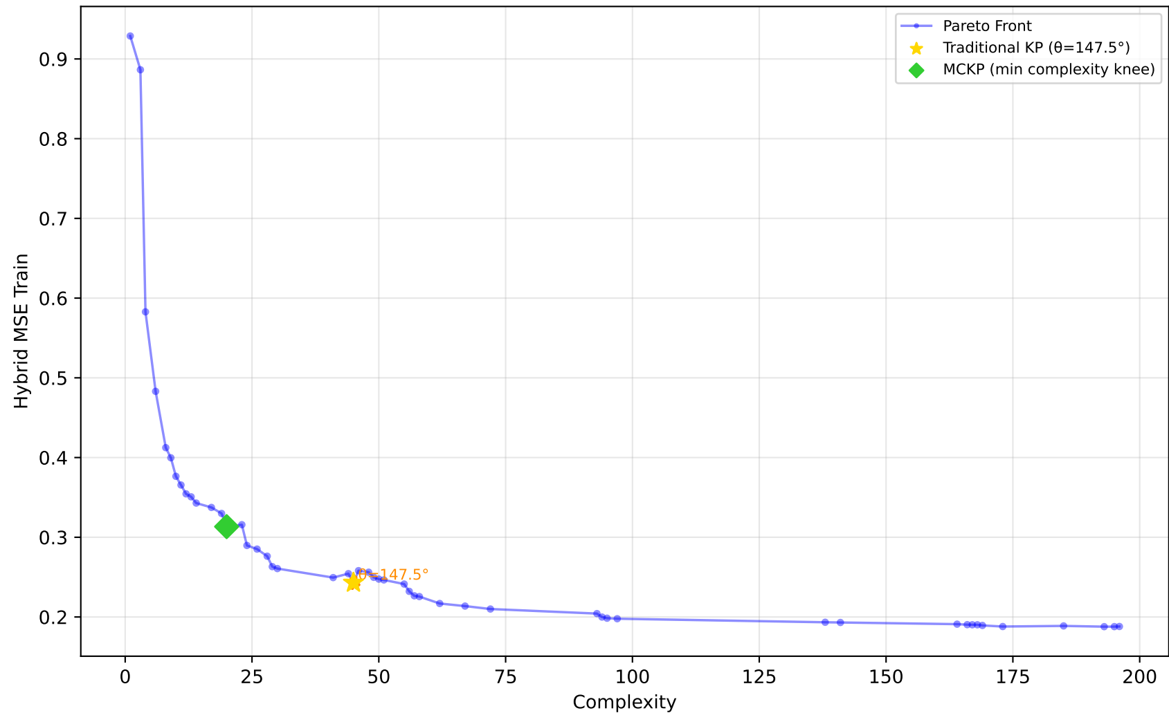
637_fri_c1_500_50 - Run 6 - SVP - Hybrid MSE Train \lambda_1=0.10, \lambda_2=0.00, \lambda_3=0.20 | Difficulty: 1.00 | Method: hmr
