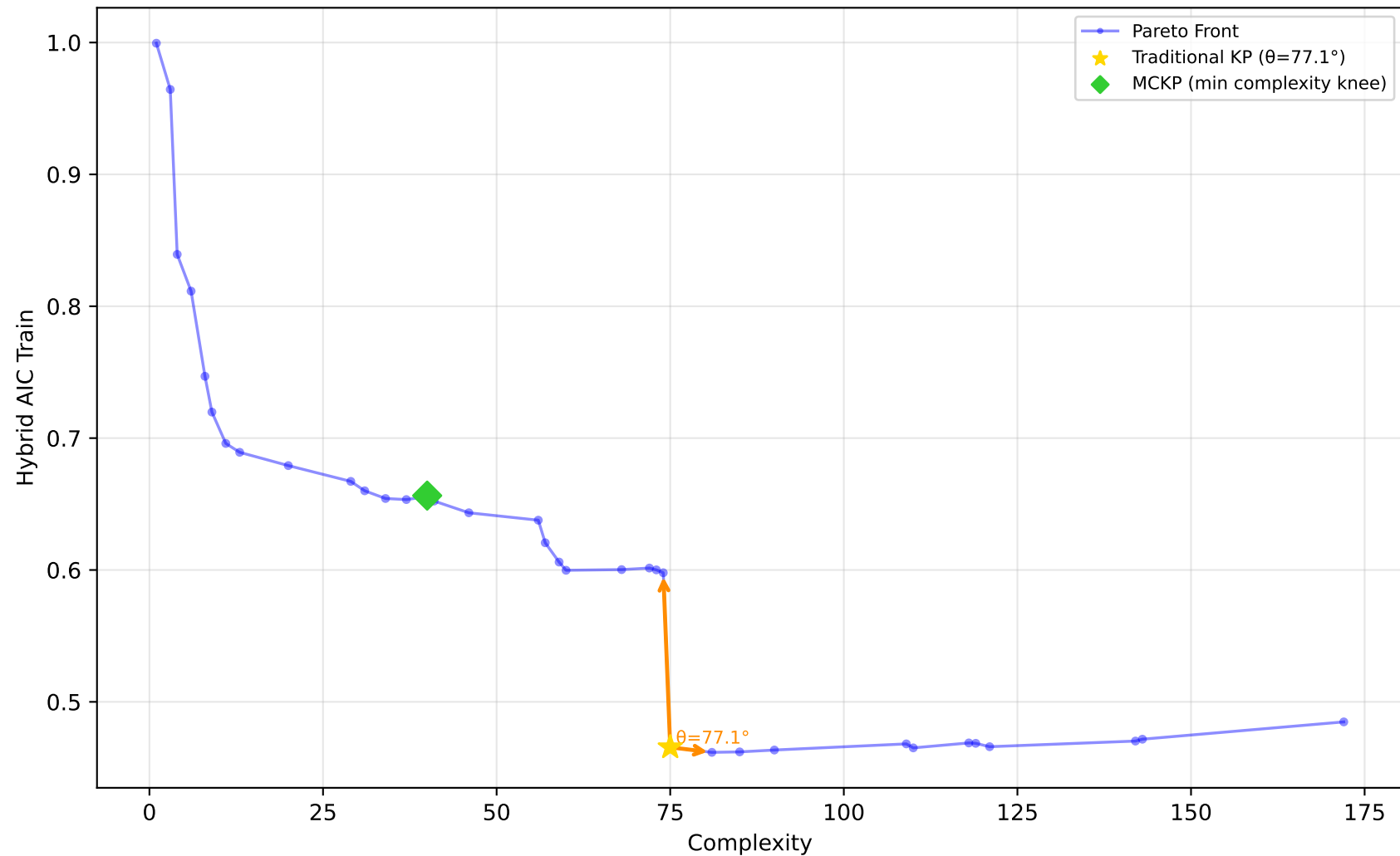
637_fri_c1_500_50 - Run 7 - MVP - Hybrid AIC Train \lambda_1=0.00, \lambda_2=0.50, \lambda_3=0.00 | Difficulty: 1.00 | Method: hmr
