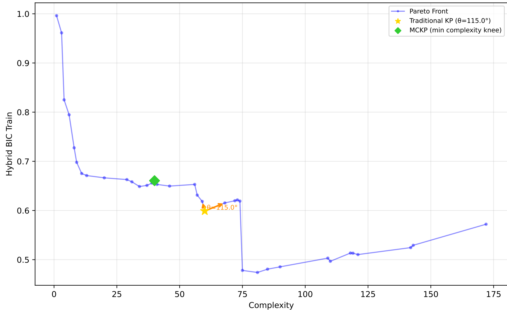
637_fri_c1_500_50 - Run 7 - MVP - Hybrid BIC Train \lambda_1=0.00, \lambda_2=0.50, \lambda_3=0.00 | Difficulty: 1.00 | Method: hmr
