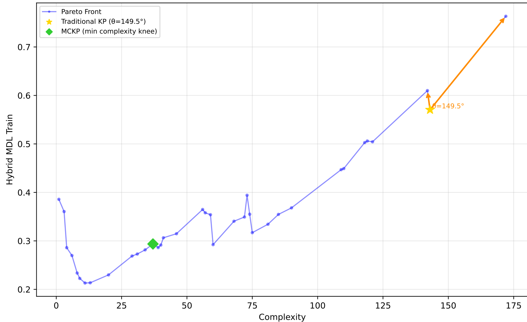
637_fri_c1_500_50 - Run 7 - MVP - Hybrid MDL Train \lambda_1=0.00, \lambda_2=0.50, \lambda_3=0.00 | Difficulty: 1.00 | Method: hmr
