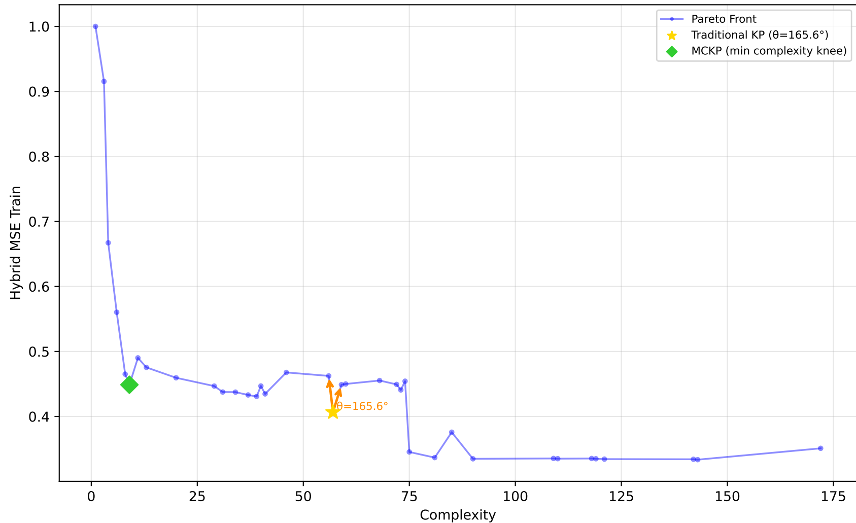
637_fri_c1_500_50 - Run 7 - MVP - Hybrid MSE Train \lambda_1=0.10, \lambda_2=0.00, \lambda_3=1.00 | Difficulty: 1.00 | Method: hmr
