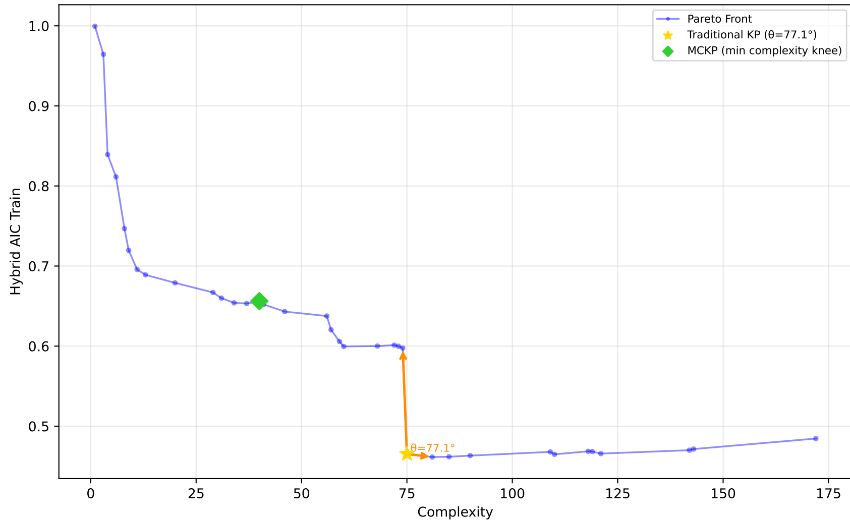
637_fri_c1_500_50 - Run 7 - SVP - Hybrid AIC Train \lambda_1=0.00, \lambda_2=0.00, \lambda_3=0.00 | Difficulty: 1.00 | Method: hmr
