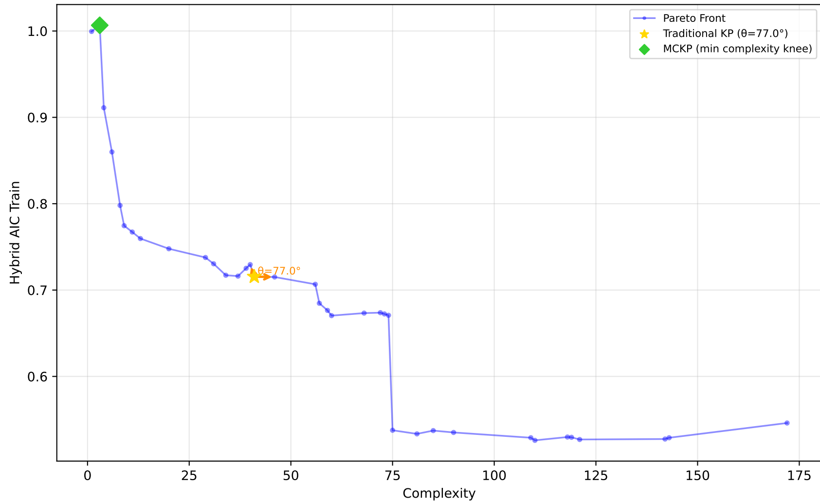
637_fri_c1_500_50 - Run 7 - SVP - Hybrid AIC Train \lambda_1=0.10, \lambda_2=0.00, \lambda_3=0.20 | Difficulty: 1.00 | Method: hmr
