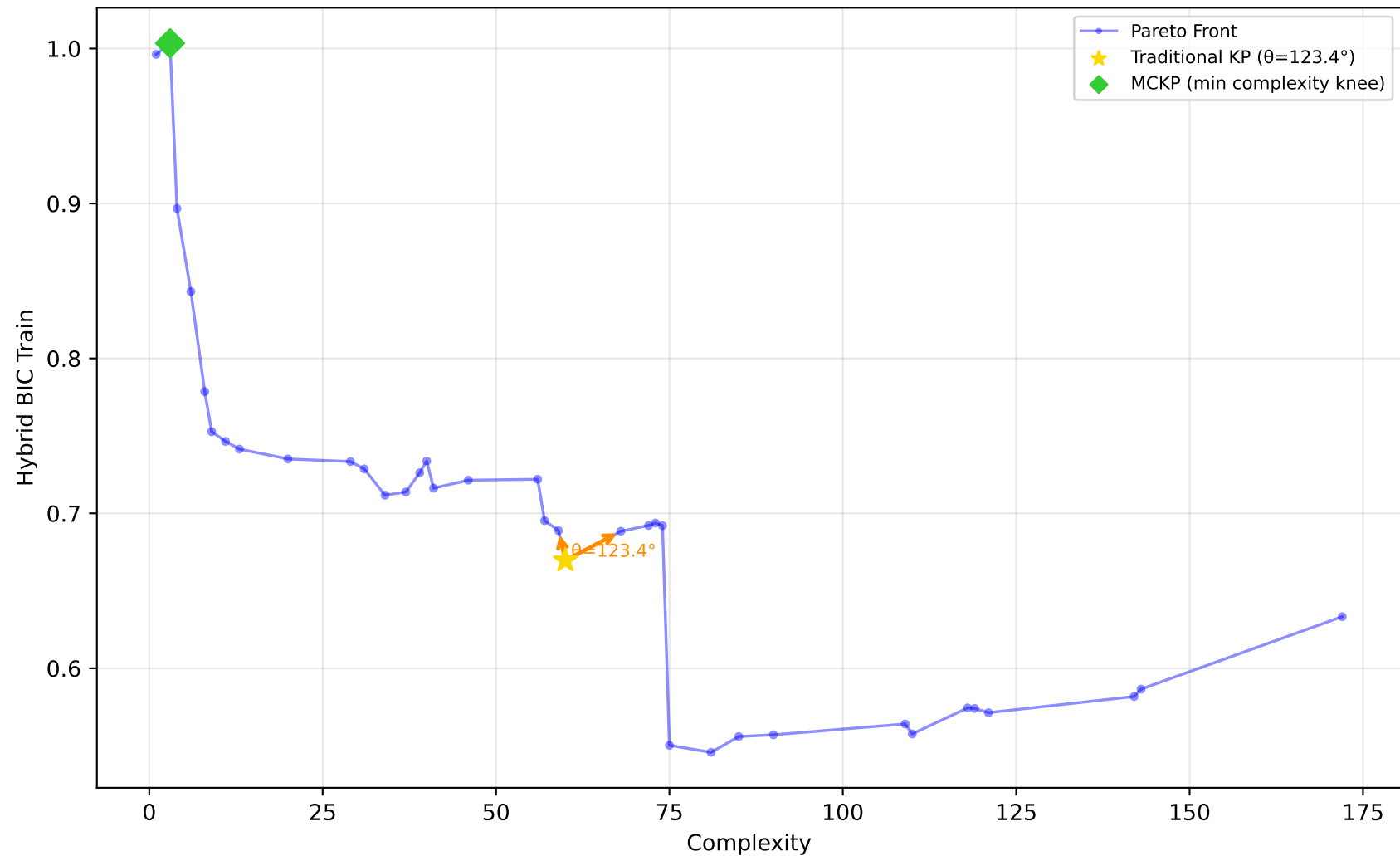
637_fri_c1_500_50 - Run 7 - SVP - Hybrid BIC Train \lambda_1=0.10, \lambda_2=0.00, \lambda_3=0.20 | Difficulty: 1.00 | Method: hmr
