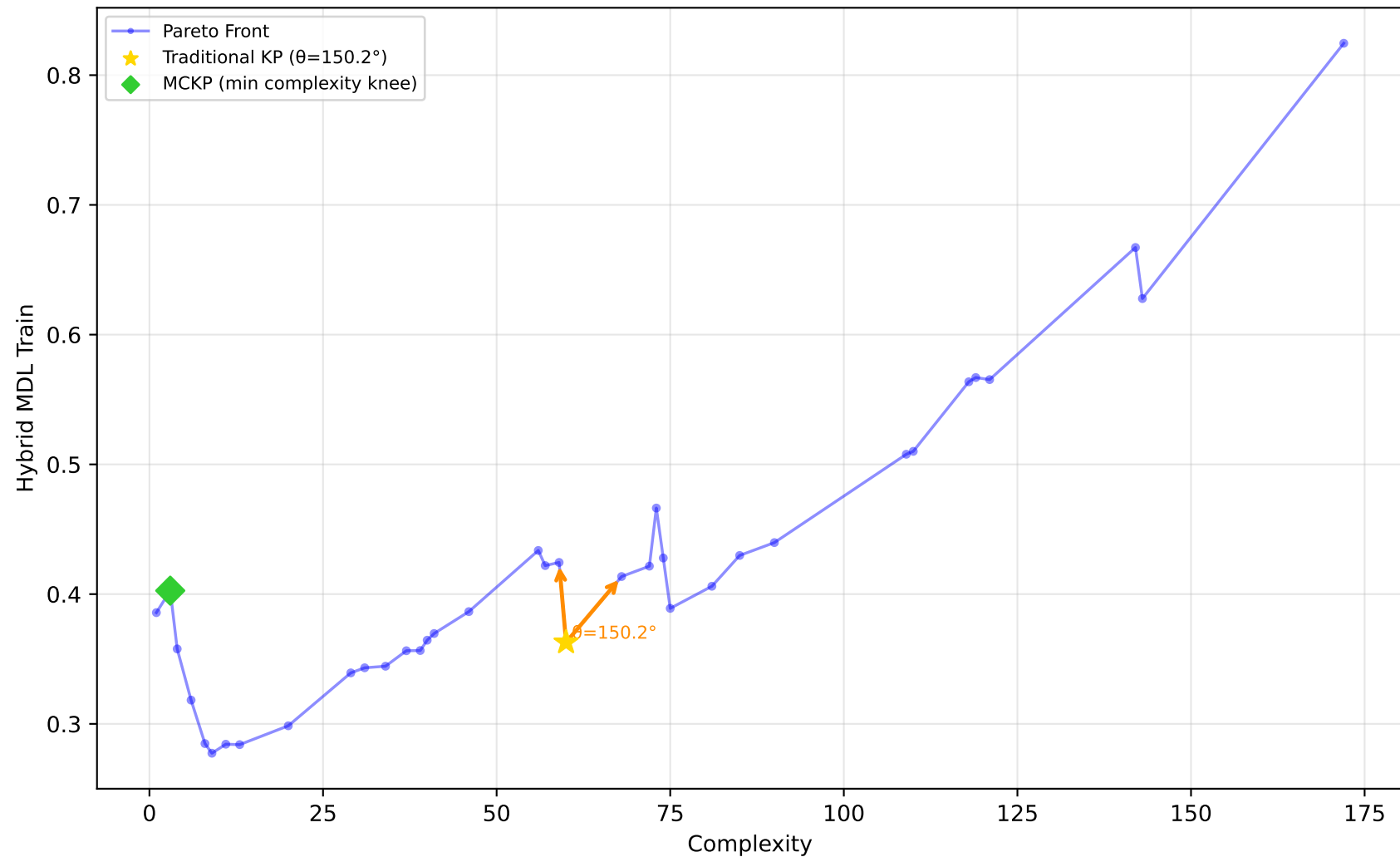
637_fri_c1_500_50 - Run 7 - SVP - Hybrid MDL Train \lambda_1=0.10, \lambda_2=0.00, \lambda_3=0.20 | Difficulty: 1.00 | Method: hmr
